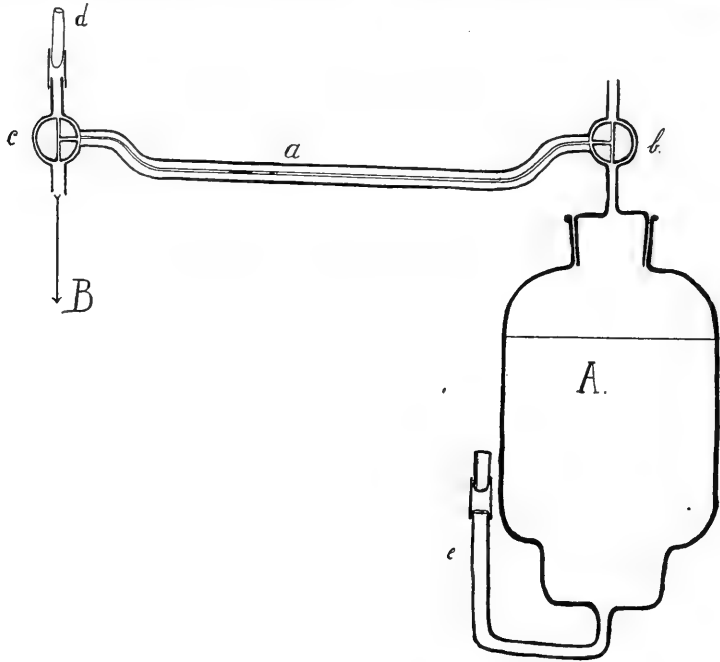
Fig. 1. Apparatus for the registration of the respiratory movements of Dytiscus .
