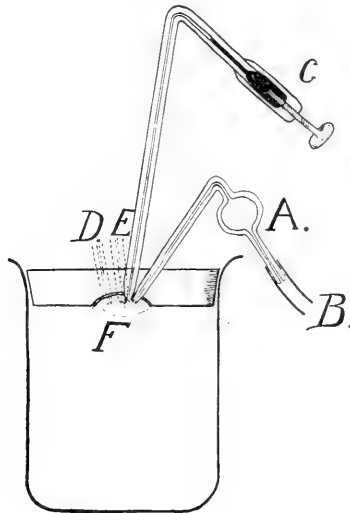
Fig. 3. Apparatus for the study of the expired air of Dytiscus . By moving a water-filled funnel connected with B upwards, the air of the bubble A is pressed into the space F , whereas the superfluous water escapes at the rim. The animal is allowed to breathe in the space F . With the pipettes C , D , and E ( D and E have been indicated with a broken line, as they do not lie in the plane of the picture) we can at every movement get a sample of the air.
