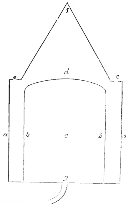
a, a, Outside 9 inch wall. b, b, Inside 4½-inch wall. c, c, Well all below ground. d, Arch. e, e, Drain-pipe. f, f, Roof. g, g, Drain.
