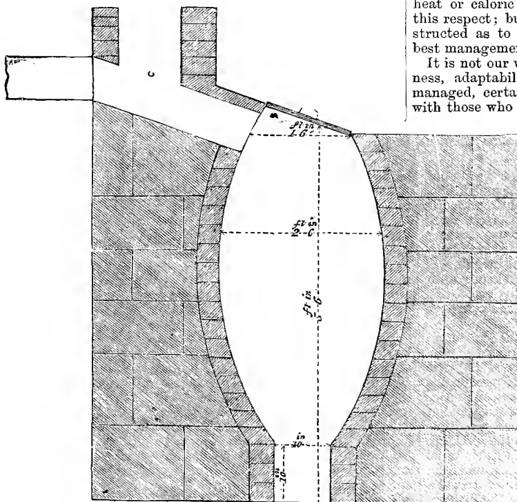
The forcing-kiln.
