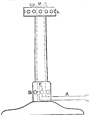
A, Gas-pipe, the jet issuing at E. B, Holes to admit excess of air. C, Apertures in the circular rim at which the gas is lighted. D, Circular lid or plate which is slid on one side when it is preferred to light the gas at the top. When the plate D closes the aperture at the top, the flame issues from the holes C in a crown, as beneath. When it is left open the flame rises in a straight jet of pale blue.
