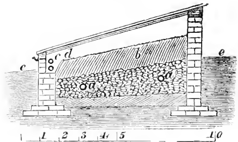
Fig. 61.—Hot-water Pit.
