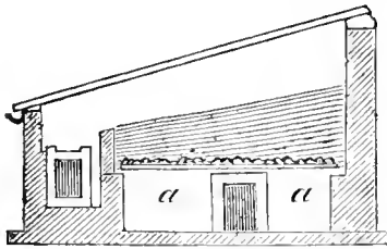
Fig. 58.—Heated Pit.
