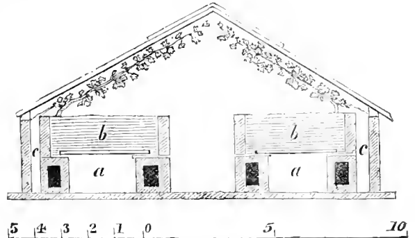
Fig. 60.—Flue-heated House.
