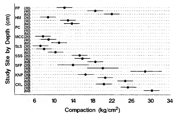
FIG. 4. Least squares means (LSMEAN ± SE) for soil compaction (kg/cm 2 ) at depths of 20, 40, and 60cm at Dakota Skipper ( Hesperia dacotae ) study sites in Minnesota, North Dakota, and South Dakota, USA (Fisher's LSD≈4.5 for n=n=4 and LSD≈7.1 for n=4, n=1; see Table 2 for study site descriptions and abbreviations, no compaction data were collected at PC, n=1 for SFP, n=4 for all other sites).
