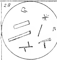
19 Cubetine chlor 210
