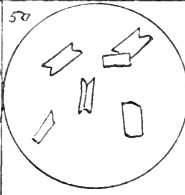
31 Scaparine alc 210
