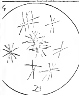
12 Rescicine alc 55
