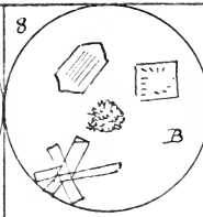
9 Codeia ether 24
