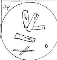
25 Quassine ether 210
