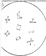
17 Colchicine water 210
