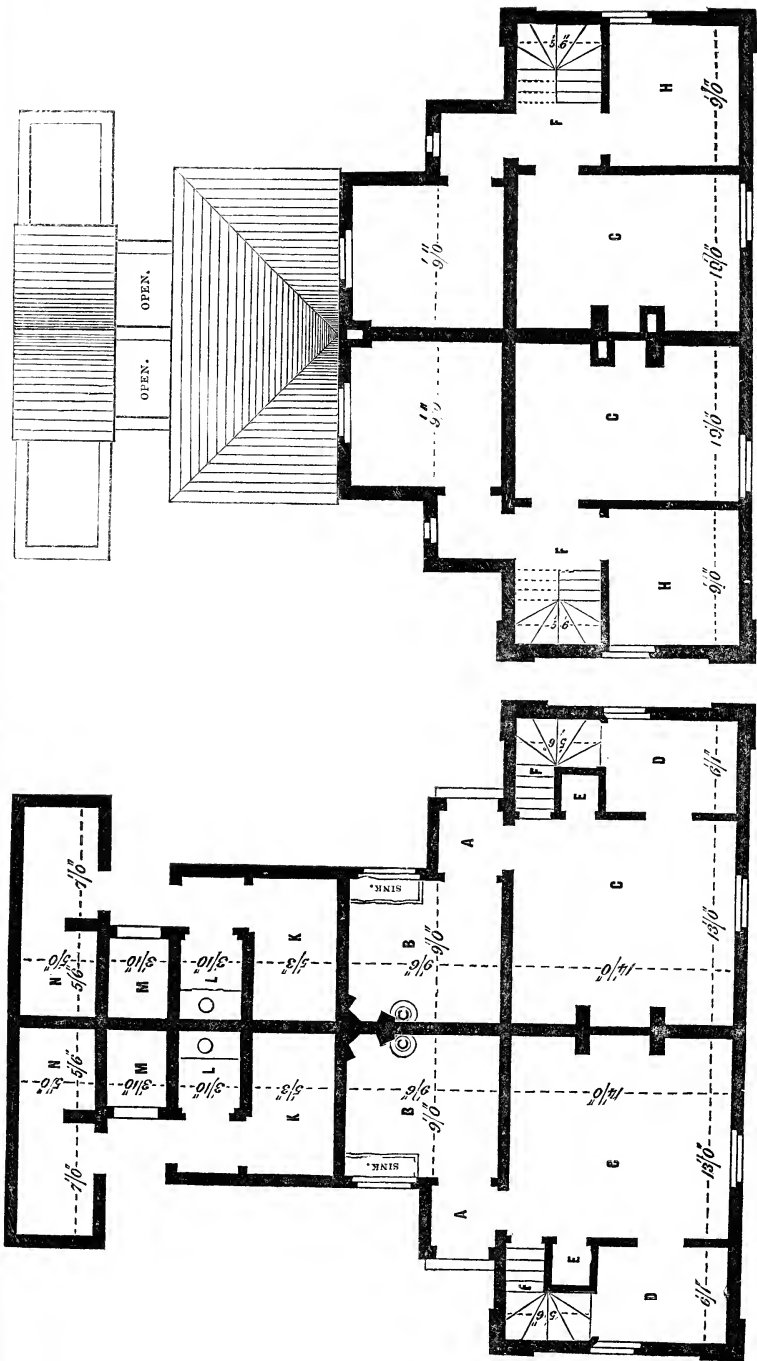
CHAMBER PLAN.
