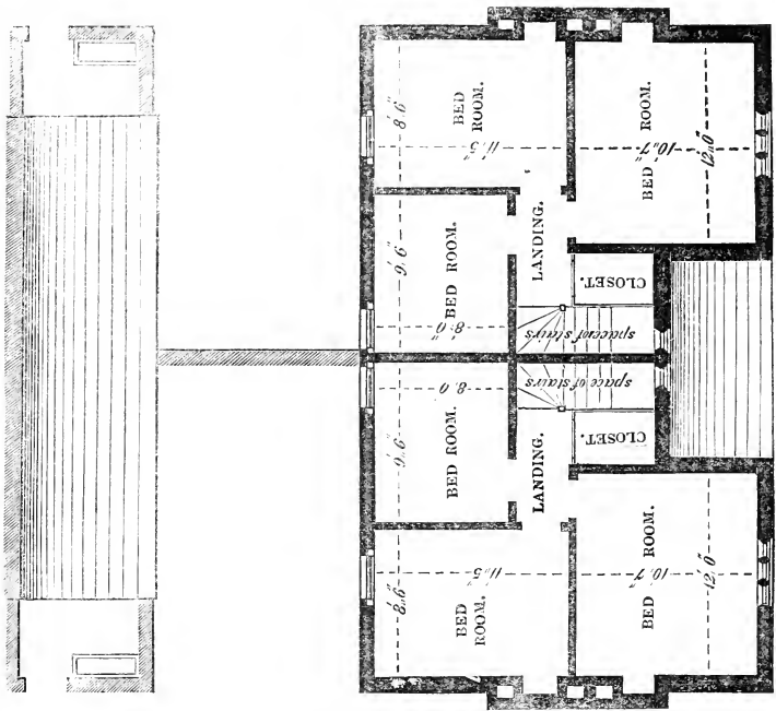
CHAMBER PLAN.
