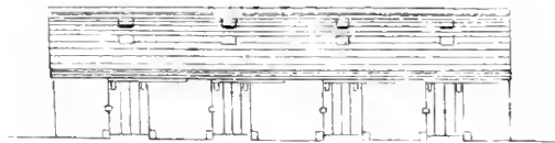
ELEVATION OF HORSE BOXES 1
