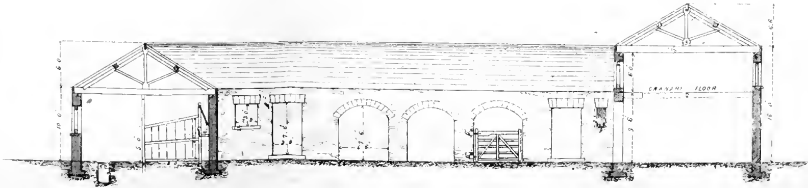
SECTION THROUGH A.B
