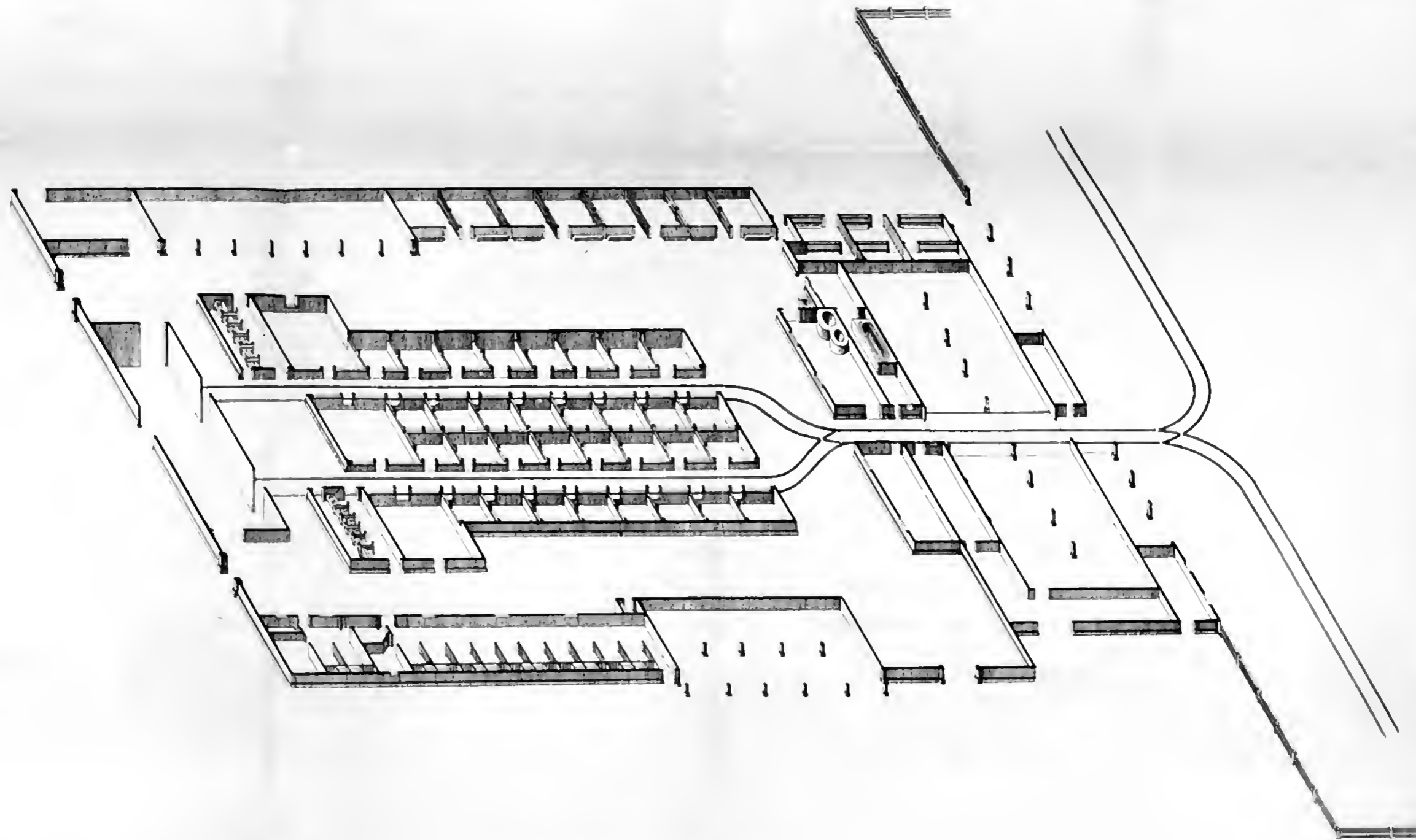
ISOMETRICAL SECTION.
