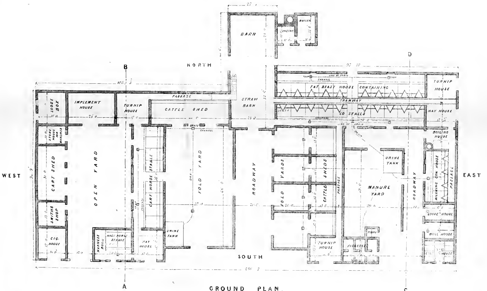
GROUND PLAN.
