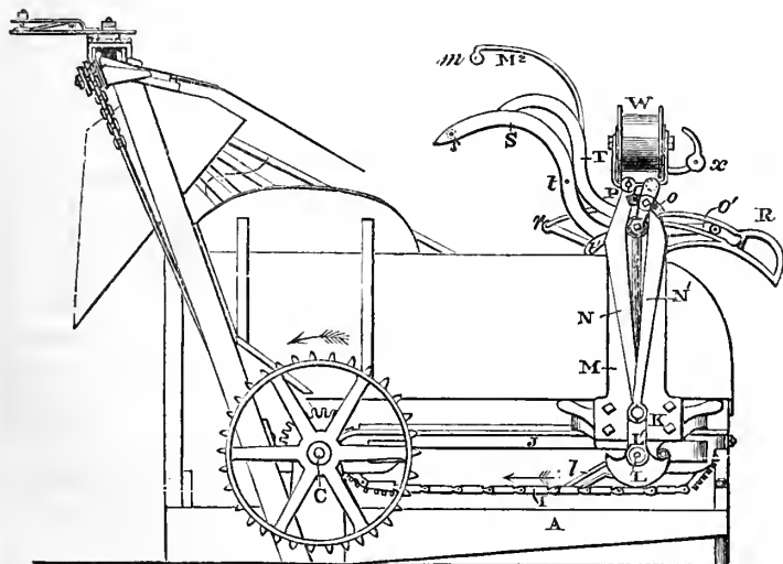
Fig. 1.— Front Elevation of McCormick's Grain-binder.
