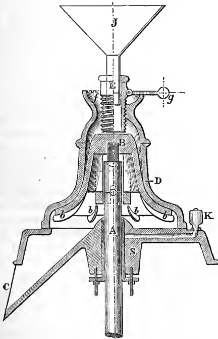
Fig. 8.—Section of Nicholson's Patent Grist Mill.
