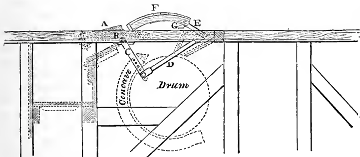
Fig. 12.—Sectional View of Messrs. Clayton and Shuttleworth's Drum-guard when closed.
