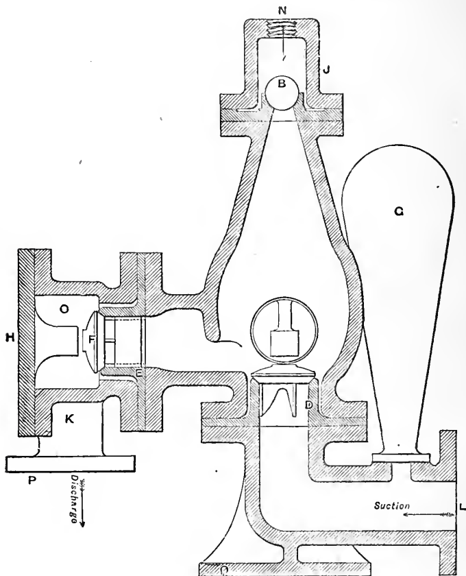
Fig. 10.— Longitudinal Section of the Hydrotrophe.
