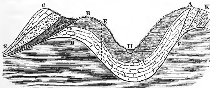
Fig. 1.— Geological Section of unconformable strata, showing Permeable Beds dipping away from the Drainage Area of their outcrop.
