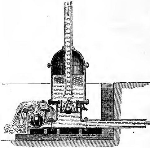
Fig. 8.— The Hydraulic Ram.
