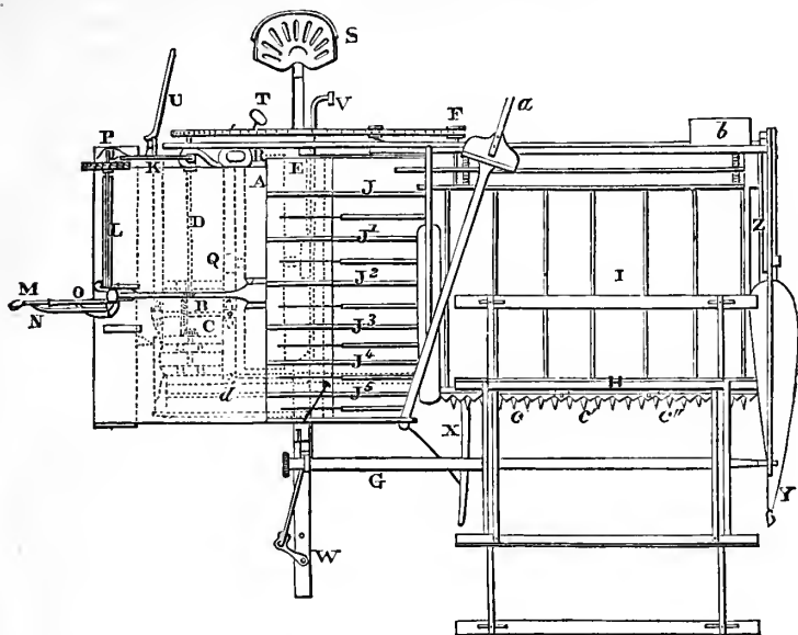
Fig. 3.—Plan of Walter A. Wood's Harvester and Self-binder combined.
