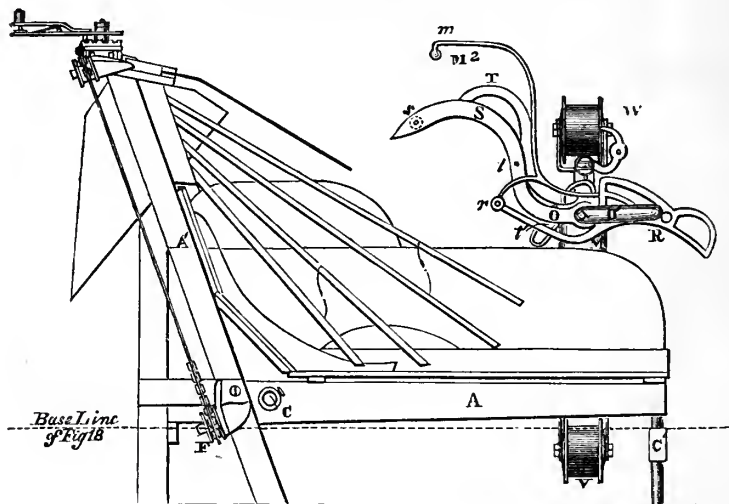
Fig. 2.—Rear Elevation of McCormick's Grain-binder.
