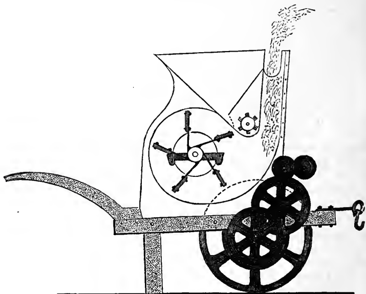
Fig. 4.—The Sulphurator.
