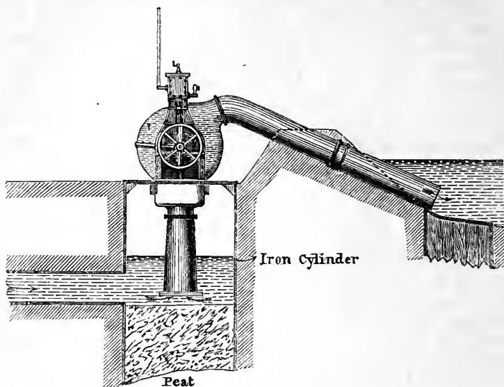
Fig. 5.—Centrifugal Pump Engine and Iron Cylinder.
