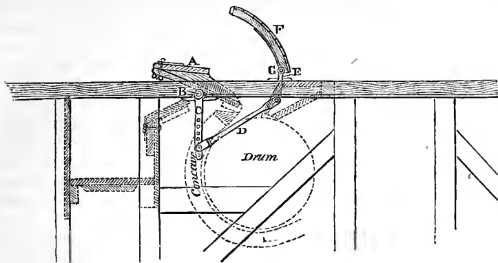
Fig. 11.—Sectional View of Messrs. Clayton and Shuttleworth's Drum-guard when open.
