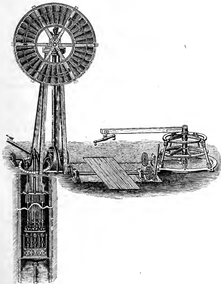
Fig. 9.— Warner's Patent Windmill, with Annular Sails, Pumps and Horse Gear.
