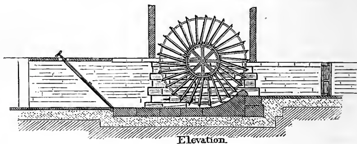
Fig. 4.— Elevation and Plan of Scoop-wheel, with Shuttle for regulating Water to it.
