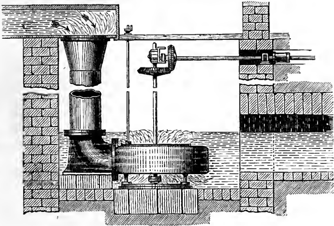
Fig. 7.— Schiele's Turbine.
