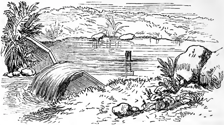
Fig. 11.—Weir, with Notch-board and Peg for measuring the Quantity of Water flowing down a Stream.
