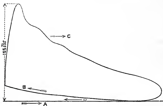
Fig. 13.—Diagram from Otto's Gas-Engine.
