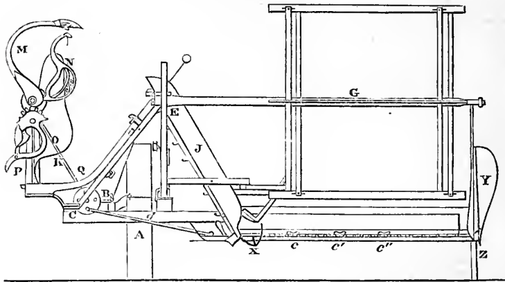
Fig. 4.— Front Elevation of Walter A. Wood's Harvester and Self-binder combined.
