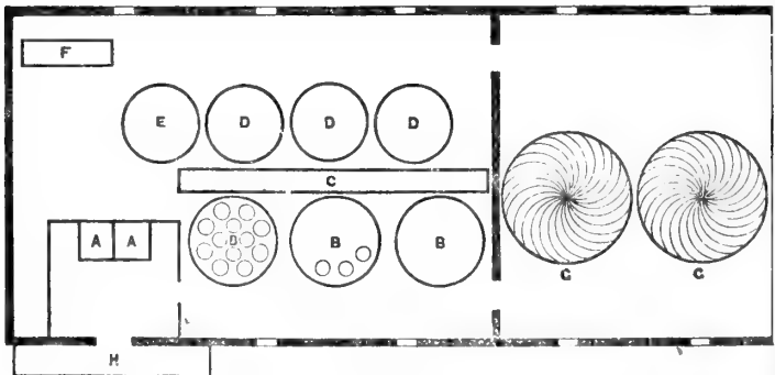
Fig. 7.— Heating-Room at Borden's Factory at Brewster.
