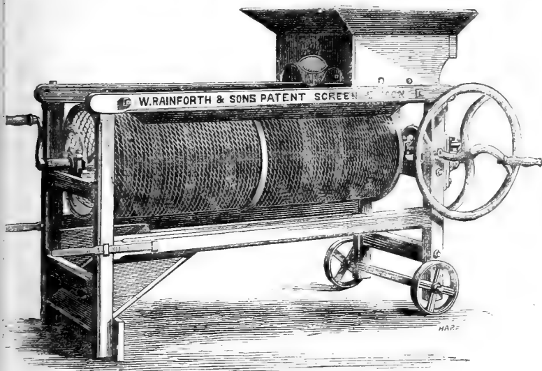
Fig. 33.— W. Rainforth and Son's Adjustable Rotary Corn Screen, No. 4152.
