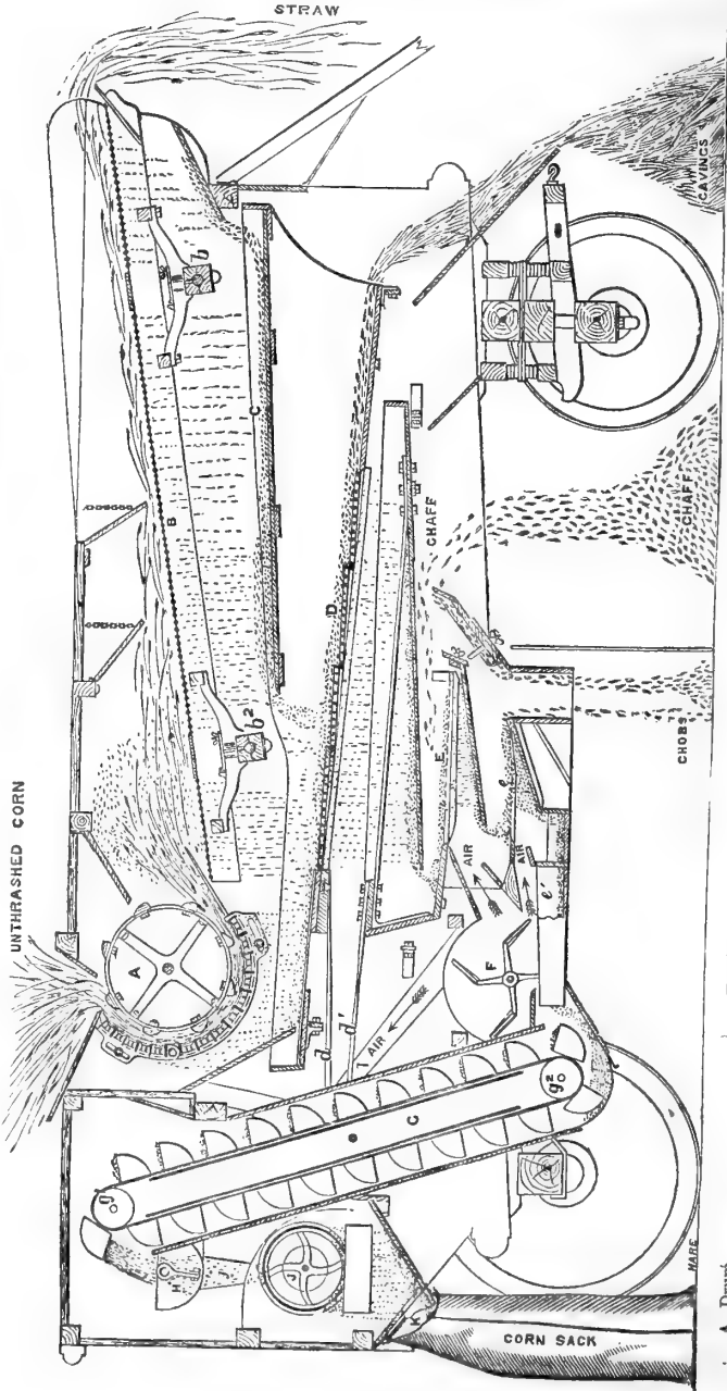
Fig. 7.—Longitudinal section of Messrs. Marshall, Sons, and Co.'s Threshing Machine, No. 5025.
