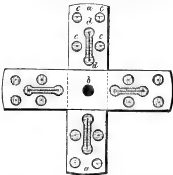
Fig. 16.—The improved Churn-Dasher (lower side).
