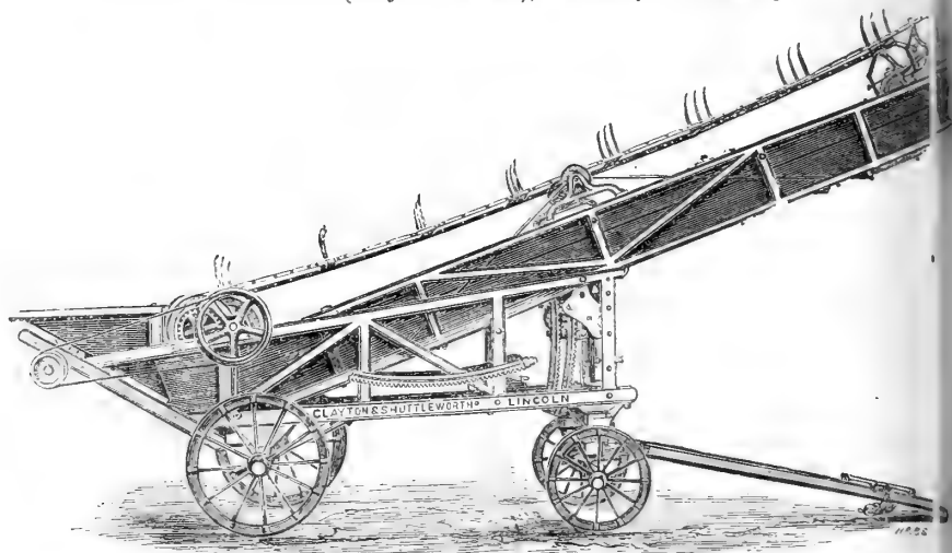
Fig. 20.—Messrs. Clayton and Shuttleworth's Improved Straw Elevator, No. 4945 (Hayes's Patent), lowered for travelling.
