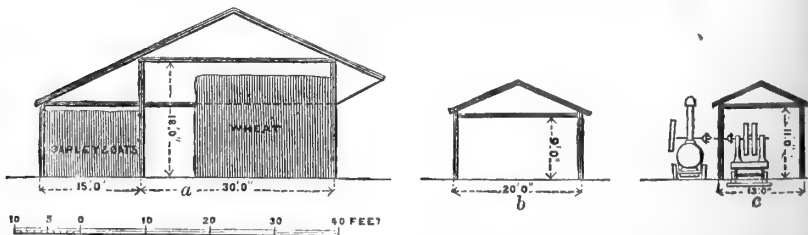
Fig. 2.—Sections of Trial-sheds and Barn at Cardiff.
