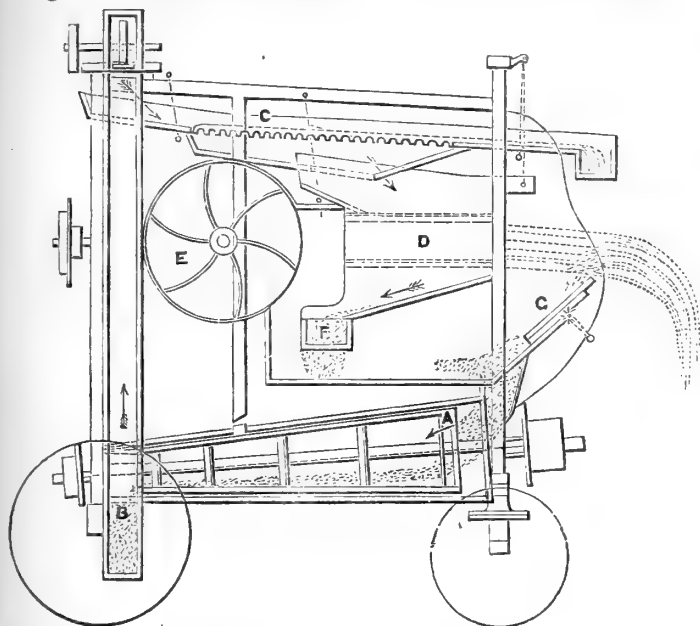
Fig. 29.—Illustrating Holmes and Sons' Seed Drawer, No. 4231.
