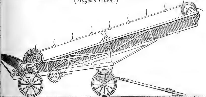
Fig. 21.— Messrs. Marshall, Sons, and Co.'s Straw Elevator, No. 5027. ( Hayes's Patent. )
