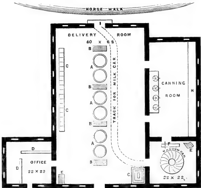
Fig. 12.—Plan of Second Floor of Middletown Milk-Condensing Factory.
