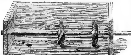
Fig. 36.— Sams's Patent Disc Seed-discharger, No. 888.
