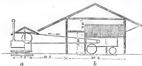
Fig. 3.—Section of Threshing-machine Shed.
