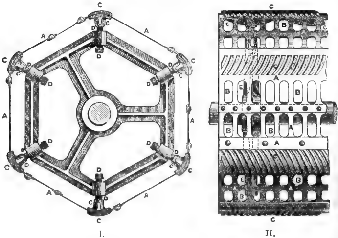
Fig. 13.—Section (I.) and Plan of part of Periphery (II.) of Brinsmead's Patent Hexagonal Drum.
