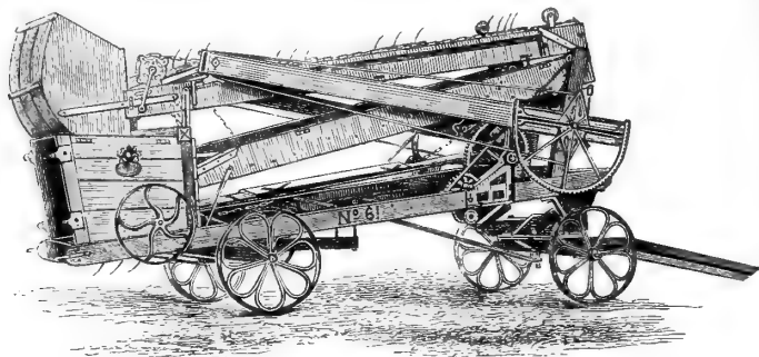
Fig. 26.— Lewin's Patent Stacker , † No. 5048, closed for travelling.
