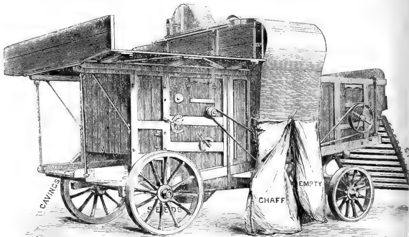
Fig. 17.—View of left side of Holmes and Sons' Threshing Machine, No. 4229.
