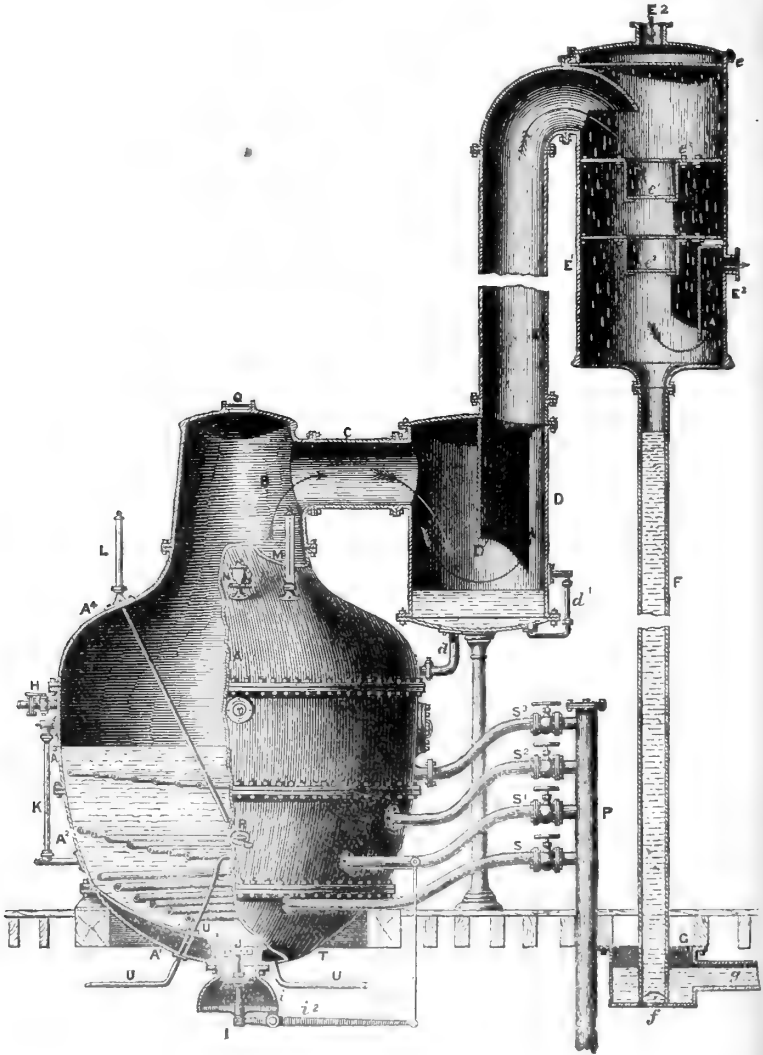
Fig. 3.— Improved Cast-Iron Vacuum-Pan.
