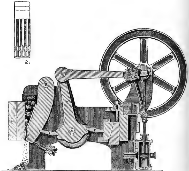
Fig. 39.—Blake's Stone-breaker.
