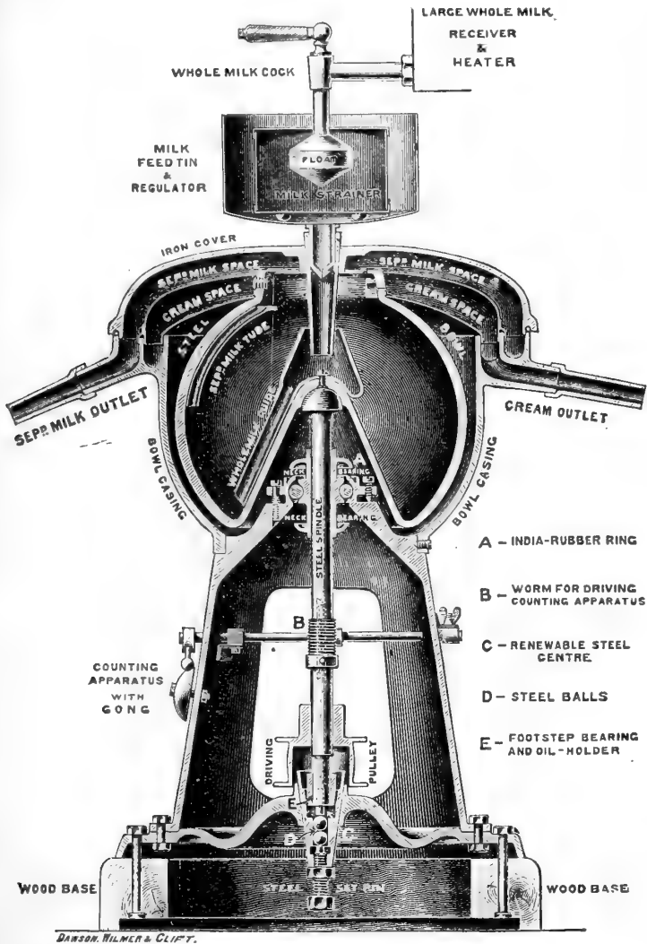
FIG. 2.—Section of "Alexandra" Power Separator.
