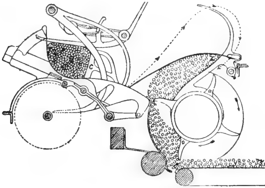
FIG. 6.—Section of the "Adriance" Binder.
