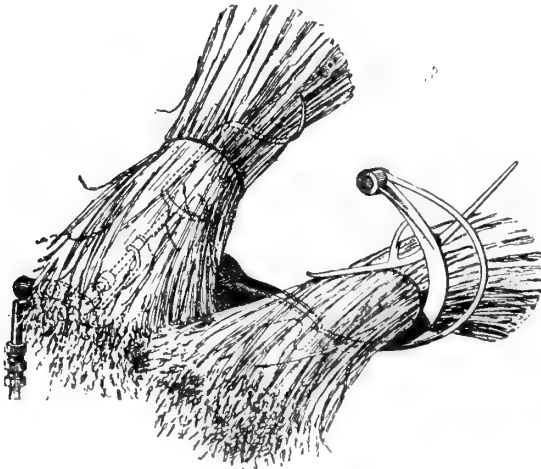
FIG. 7.—Discharger-fork of the "Adriance" Binder. The dotted line shows the centre of motion in turning the bundle.
