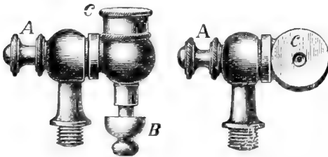
FIG. 15.—The Vermorel nozzle.
