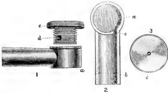
FIG. 16.—The Riley nozzle.
