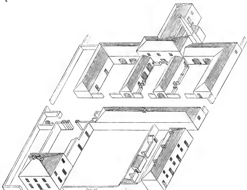
AN ISOMETRICAL PROJECTION of the FARM-HOUSE and FARMERY represented in Plan No. 1.
