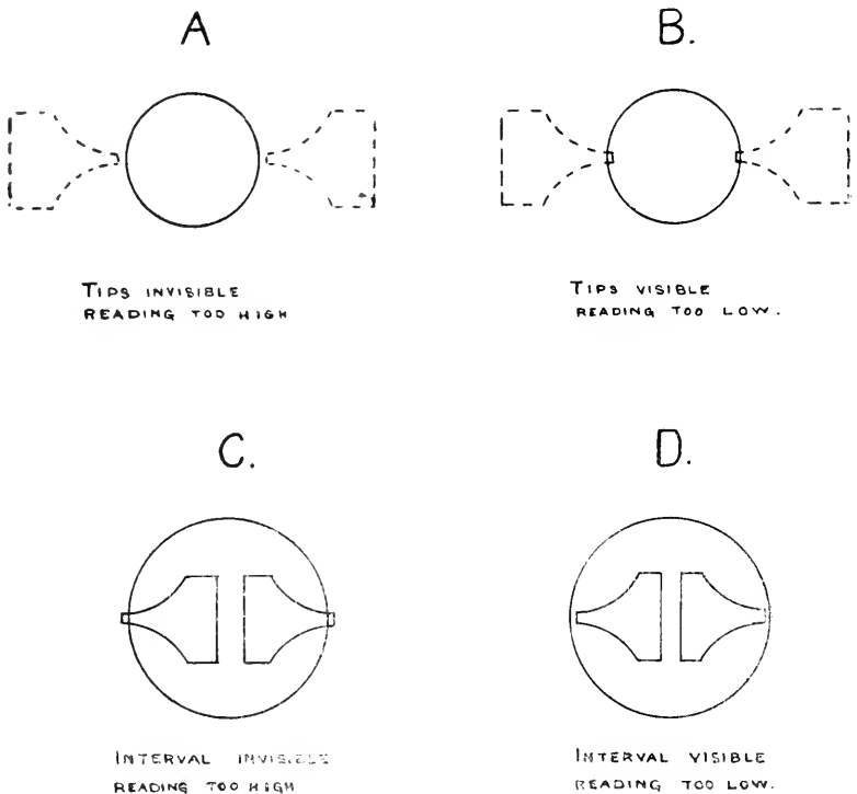
FIG. 1.—Diagrams to show how error is caused by the restriction of the visible field to the aperture of the objective.
