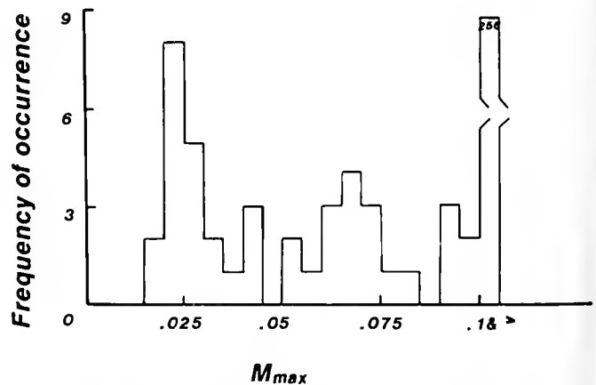
Figure 2a. Estimates of \hat{M}_{max} derived from survival of tagged scallops, calculated from weekly recoveries. Figure 2b. Estimates of \hat{M}_{max} derived from short-term survival data.
