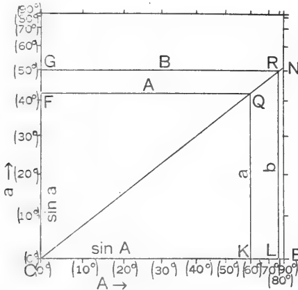
Fig. 4. Straight line sine diagram for the solution of the sine formula of spherical trigonometry. This chart, which has long been used, is the northeast quadrant of plate I and is based on the relation \sin a : \sin b = \sin A : \sin B . In fig. 4 QK = \sin a , OK = \sin A , RL = \sin b , OL = \sin B . If any three of these four elements are known, the fourth can be read off directly from the diagram by virtue of the similar triangles OQK and ORL .
