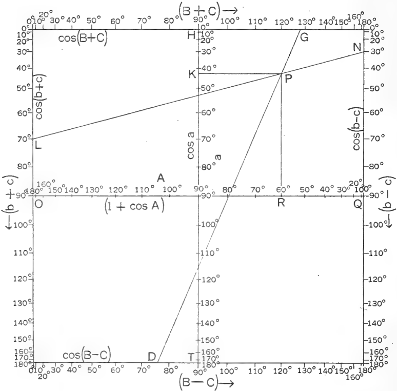
Fig. 3. Straight line cosine diagram for the solution of any spherical triangle in which any three of the six elements are given. In this chart the scales on the horizontal lines refer to the angles A, B, C ; the scales on the vertical lines refer to the sides a, b, c . In case two sides and the included angle or the third side are given the construction described under fig. 1 is used; if two angles and the included side or the third angle are given, the construction of fig. 2 is followed except that in this diagram the axes of fig. 2 have been rotated through 90^\circ , as indicated by the labeled scales. For the case that two sides and an opposite angle or two angles and an opposite side are given, it is necessary first to find the second opposite angle of the second side by the use of the sine chart (fig. 4) and to plot the lines LN and DG , the intersection P of which determines the remaining angle and side simultaneously.
