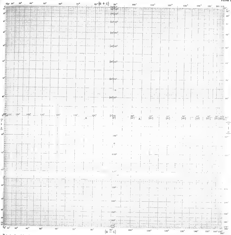
Plate 1. On this plate, which is a reproduction of sheet No. 2776 of the U. S. Hydrographic Office but with relabeled and additional scales, the scales of figs. 3 and 4 have been combined into one diagram, which is made to serve both as a cosine chart and as a sine chart, thus rendering it capable of solving any spherical triangle in which any three of the six elements are given; sought are the three remaining elements. The mode of construction depends on the elements given. For the six possible cases the constructions are described in the text and also under figs. 1 to 4.
