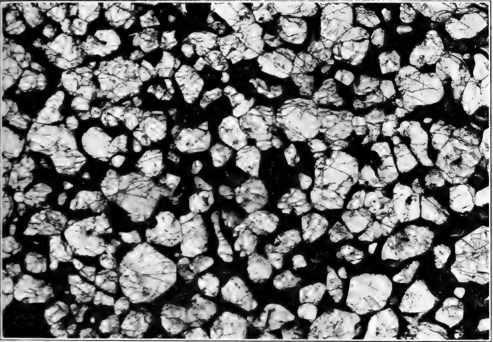
Fig. 4. Actual lithospor (meteoric). Photograph of section of Mount Vernon pallasite. The iron is shown as black.
