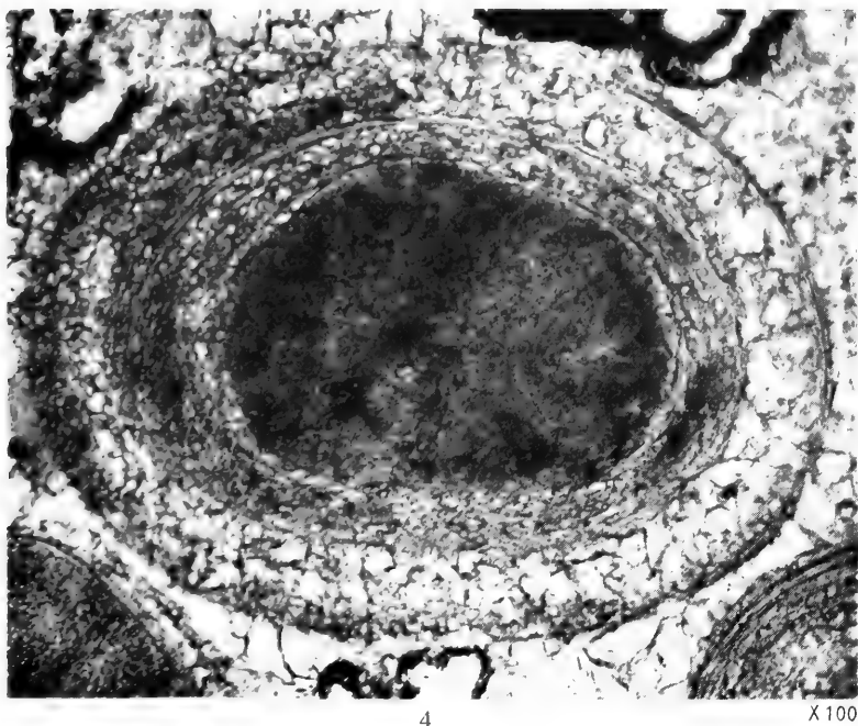
Figs. 1, 2, 3. Thin sections of ellipsoidal grains from muds. Figs. 1, 3, b.s. 261, Bahamas, Fig. 2, b.s. 88, Bahamas. Fig. 4. Thin section of oolite grain, Bahamas.
