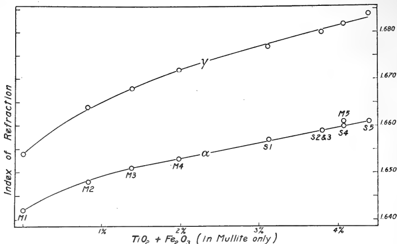
Fig. 1.—Relation between the refractive indices of various mullites and sillimanites. M1, M2, etc. = mullite I, mullite II etc. of Table 5. S1, S2, etc. = sillimanite I, sillimanite II, etc. of Table 6.
