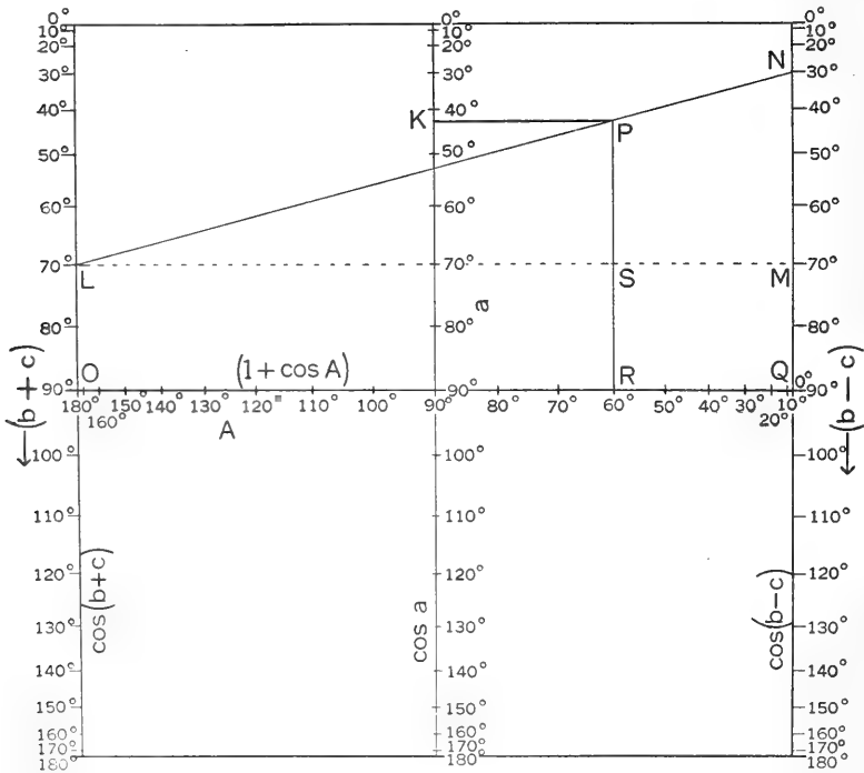
Fig. 1. Straight line cosine diagram for the graphical solution of a spherical triangle in which two sides b, c and an included angle A or the third side a or the included angle A . Pass a straight line through the points L [angle (b+c) ; distance LO = \cos(b+c) ] and N [angle (b-c) ; distance NQ = \cos(b-c) ]; intersection P of this line with the ordinate erected at R [angle A ; distance OR = 1 + \cos A ; or angle a ; distance PR = \cos a ] is the desired point P which determines A and a .
