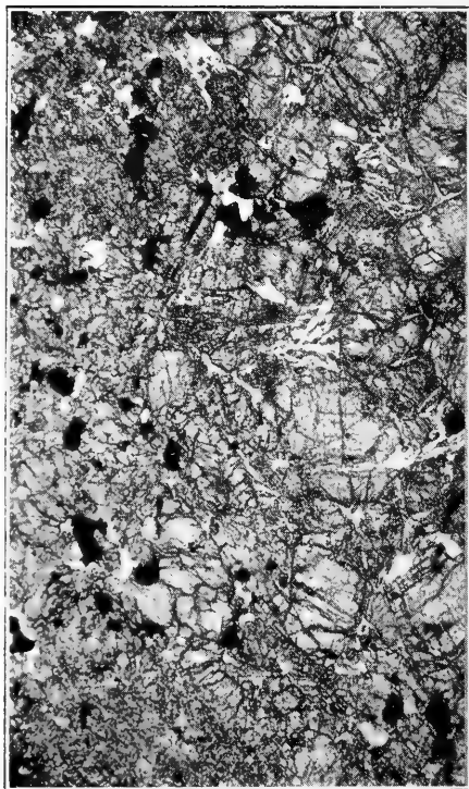
Fig. 5b. Actual ferrospor (meteoric). Photograph of section of the Alfianello stony meteorite. The iron is shown as black.
