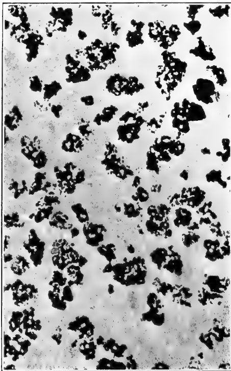
Fig. 5a. Actual ferrospor (terrestrial). Photograph of section of iron-bearing basalt from Kaersut, West Greenland. The iron is shown as black.
