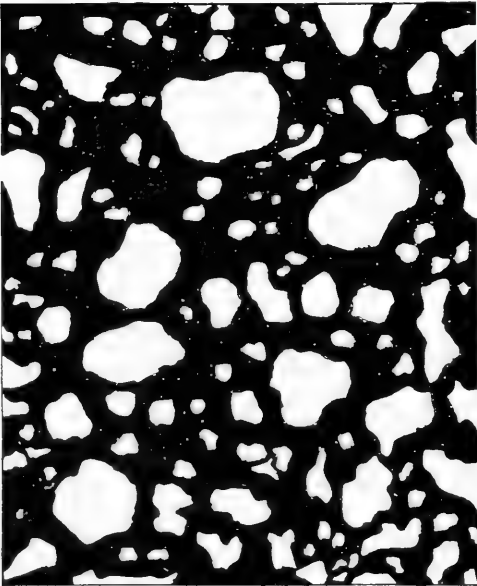
Fig. 2. Diagrammatic representation of a lithospor: silicate scattered, or sporadic, in a continuum of iron.
