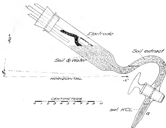
Fig. 1. The filled electrode vessel.
