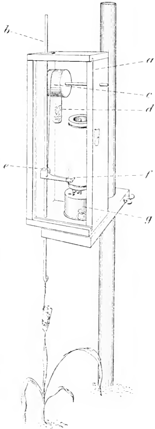
Fig. 1. Field auxanometer.
