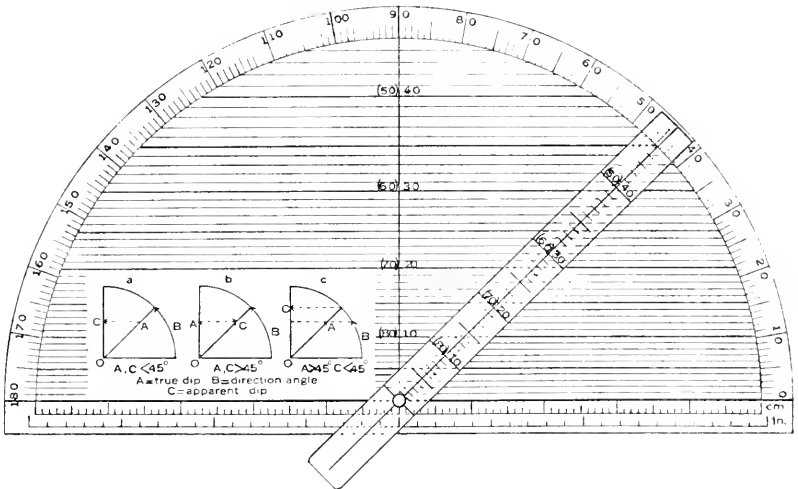
Fig. 1. A geological protractor.
