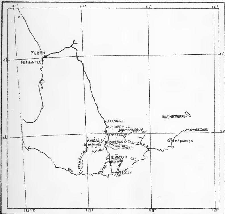
Fig. 1. General locality map showing the relation of the Stirling Range to the Porongrupps and to the Frankland-Gordon and Pallinup River Systems.
