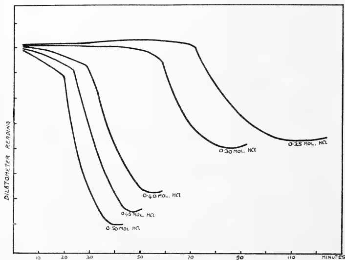
Fig. 2. Sodium nitrite (1 mol.), aniline hydrochloride (1 mol.) and hydrochloric acid. Temperature: 9.5^{\circ} C.
