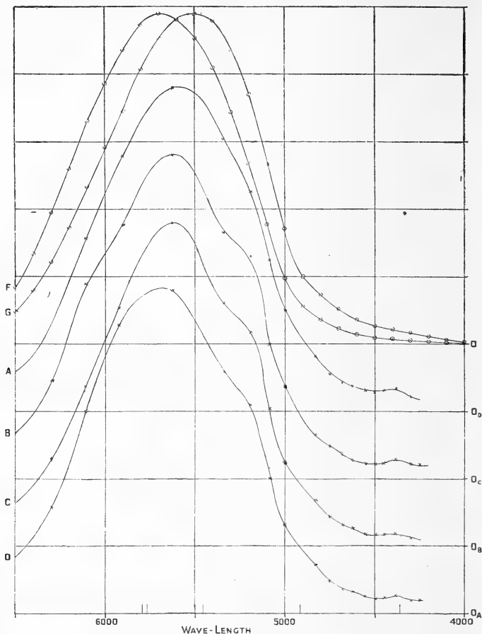
Fig. 2.—Luminosity distribution curves. The letters A, B, C, D, F, G refer to the tubes A, B, C, D, and black bodies at 3,000^{\circ} and 6,000^{\circ} respectively, the origins being again separated except in the case of the two black bodies. The units have been arbitrarily chosen to make all the values equal at \lambda 5600 .
