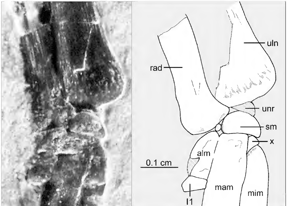
Fig. 15. Photograph and interpretive drawing of the carpus and manus of GMV-2158. Abbreviations: sm, semilunate carpal; unr, ulnare; x, carpal X; II, proximal phalanx of alular digit. Other abbreviations as in figure 3.
