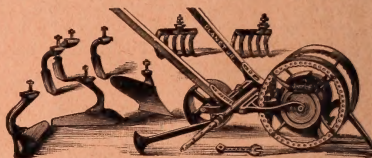
The "Planet Jr." Combined Drill, Wheel Hoe Cultivator and Plow. Price, $8.50.
