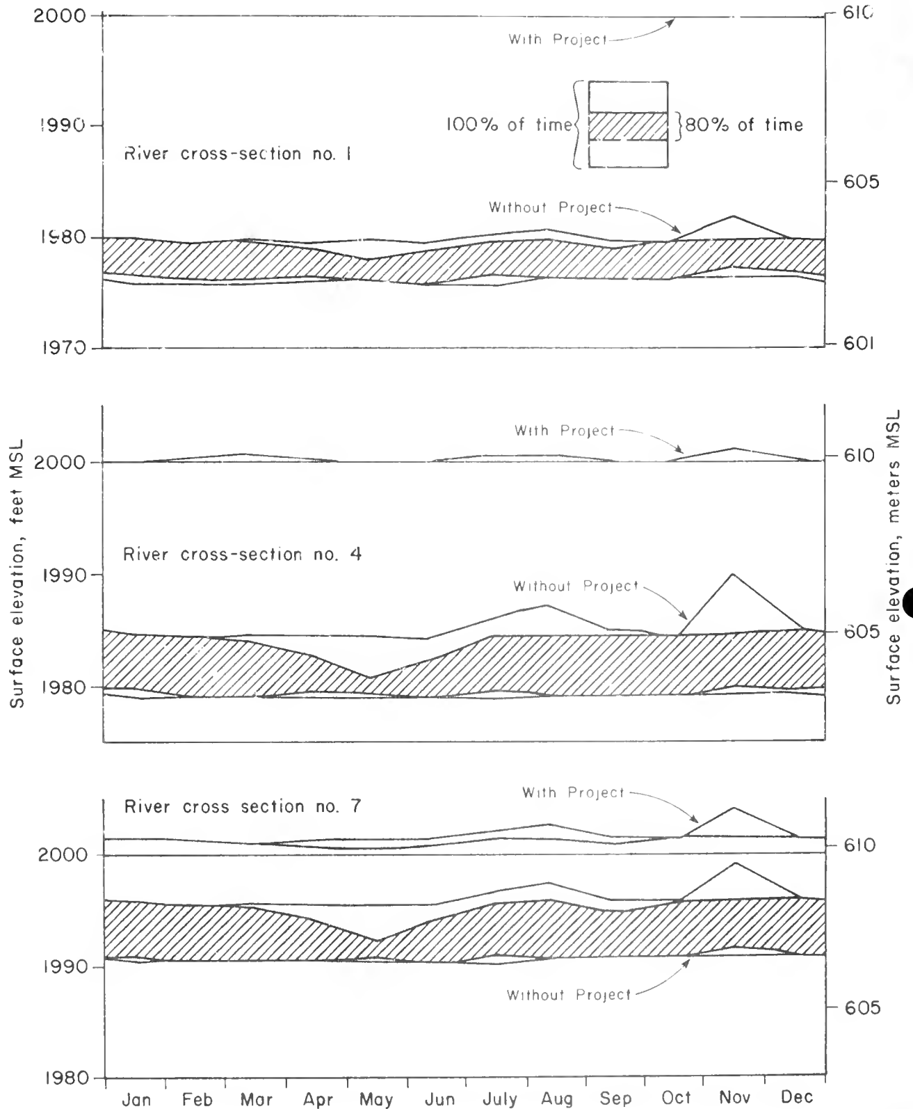
FIGURE 13. Typical seasonal variation in surface elevation of the Kootenai River at three river cross sections, with and without the proposed dam, assuming a forebay elevation of 610m (2,000 ft) and the pattern of discharge shown in Figure 12 (SOURCE: Sewell and Associates 1979).
