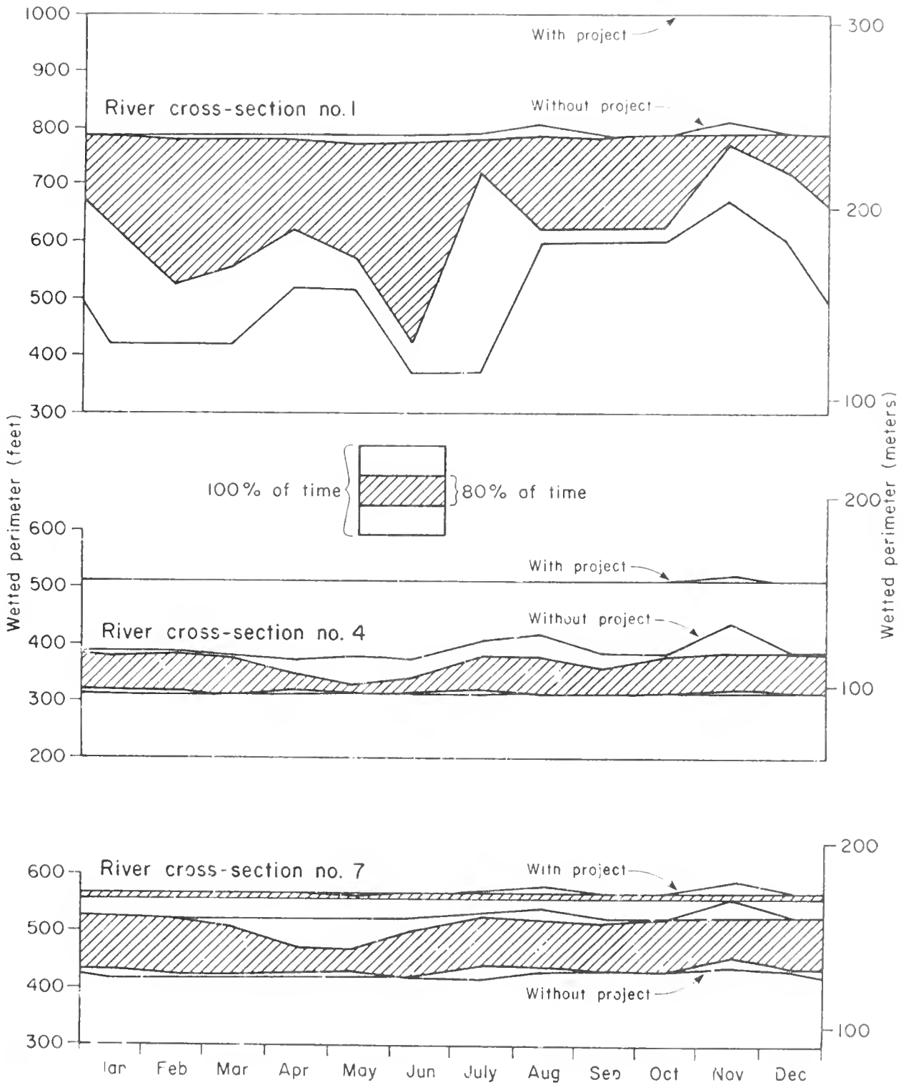
FIGURE 14. Typical seasonal variation in wetted perimeter and width of littoral zone (area between daily high and low water marks) of the Kootenai River at three river cross sections, with and without the proposed dam, assuming a forebay elevation of 610 m (2000 ft) and the pattern of discharge shown in Figure 12 (SOURCE: Sewell and Associates 1979).
