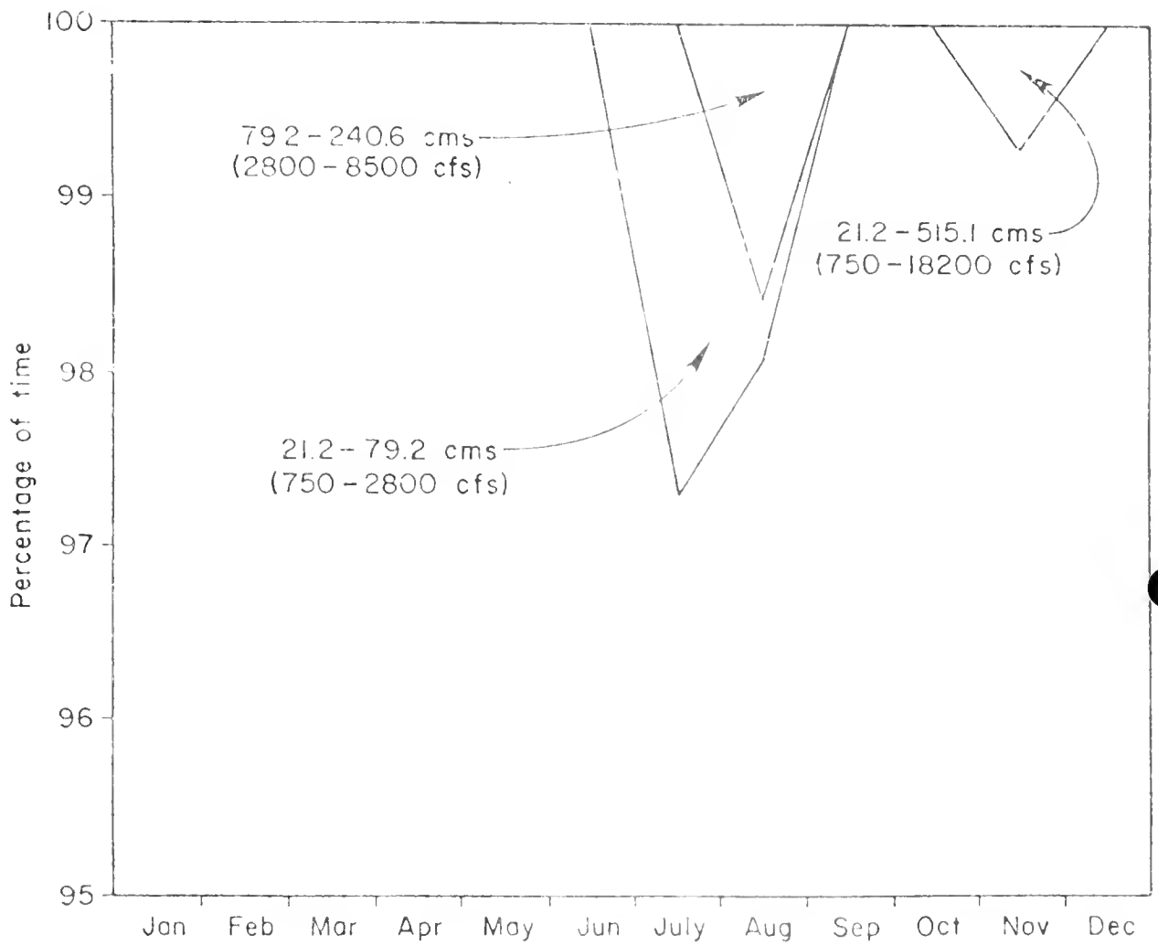
FIGURE 16. Percent of time that different flows would be allowed to pass over the Kootenai Falls Dam. (SOURCE: Sewell and Associates 1979).
