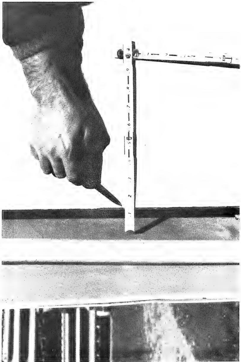
Figure 11. Gap between the generator frame and end of the generator blade.
