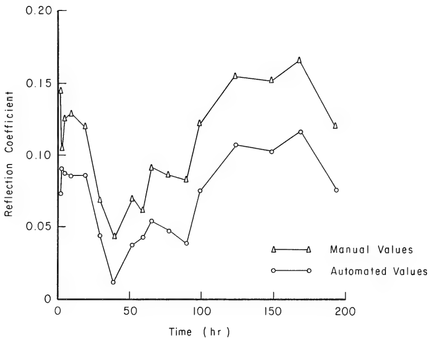
Figure 15. Lower K_R values and similar K_R trend from automated method in experiment 70X-10.
