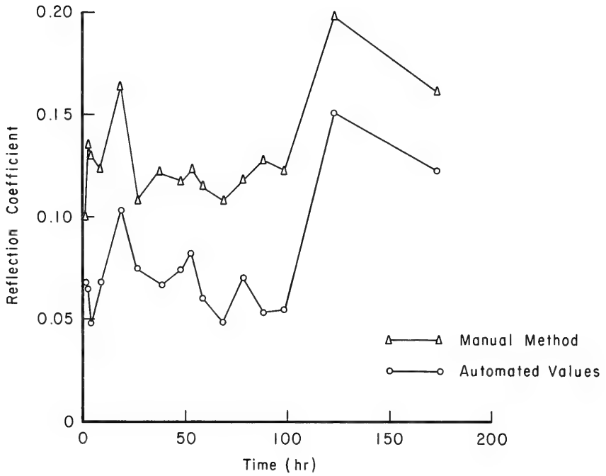
Figure 14. Lower K_R values and similar K_R trend from automated method in experiment 70X-06.
