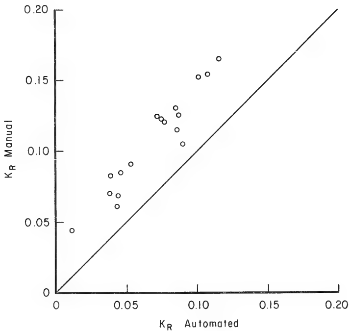
Figure 17. Correlation of manual and automated methods for determining K_R (experiment 70X-10).
