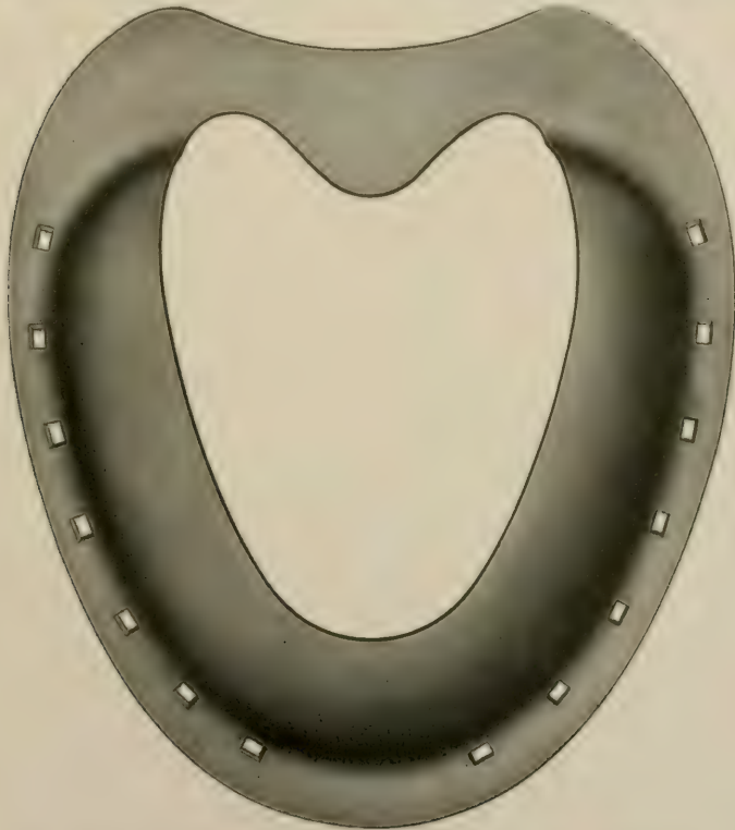
Fig. 36—Superior surface, showing concavity or bowl, as formed by the toe and branches of the shoe, as designed by Dr. David W. Cochran.
