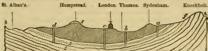
SECTION ACROSS THE LONDON BASIN FROM ST. ALBAN'S TO KNOCKHOLT.
