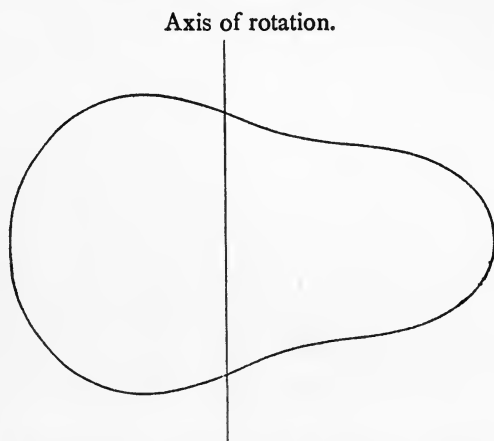
FIG. 8. Poincaré's pear-shaped figure of equilibrium.
