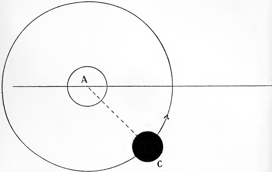
FIG. 10. Algol and relative orbit of companion.
