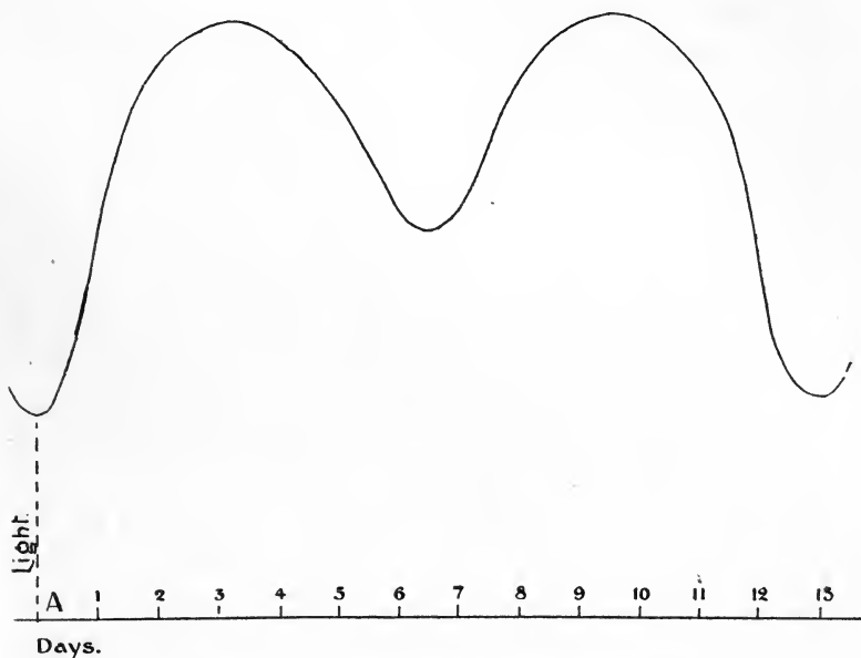
FIG. 13. Light Curve of \beta Lyrae.
