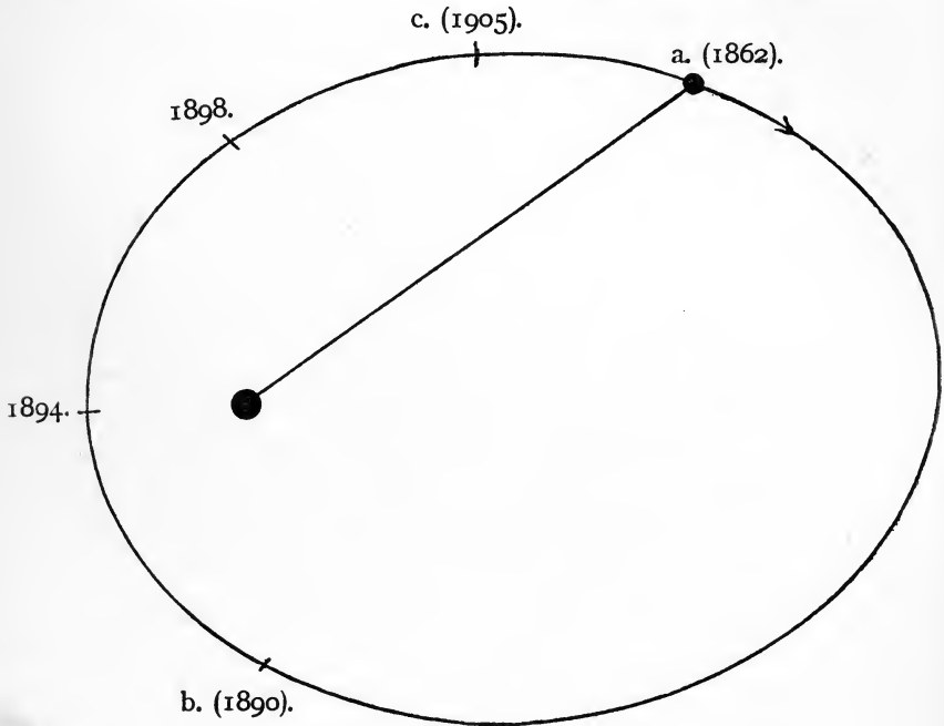
FIG. 3. Sirius, and relative orbit of companion.
