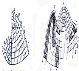
Fig. 78. Diagram of a growing point in longitudinal section. The right hand half represents a later stage in the development of the left hand half.
