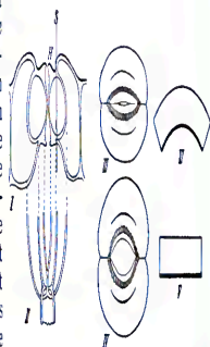
Fig. 8. I-IV, stoma of Amaranthus ferrocristatus after SCHWENBENER. I, in section; II, surface view of closed stoma; III, surface view of a closed, and IV, of an open stoma; V, VI, for explanation see text.
