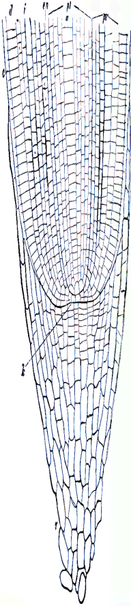
Fig. 86. Median longitudinal section of the root apex of Hieracium vulgare . i , initial cells of the root cap; r , cells of the cap about to be thrown off; c , central cylinder; an , endodermis; e , intercellular spaces; ep , epidermis; e , thickened external wall of the epidermis. From STRASBURGER ( Das botanische Praktikum , 4th ed., Jena, 1906).
