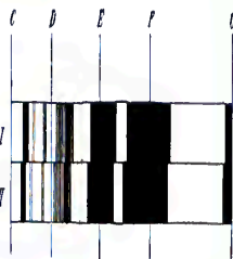
Fig. 25. Absorption spectra. I of phytyloporphyrin (in ether); II of haematoporphyrin (in ether). After MARCHEWSKI, in ROSCOE and SCHROEMMER'S Lehrbuch der Chemie , vol. VIII, 1901.
