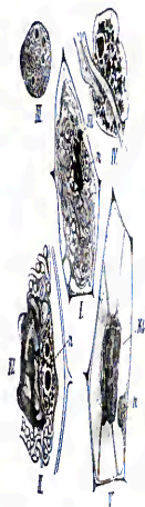
Fig. 44. Polium triquetrum . I, Cell of the root filled with fungal hyphae; II, nucleus; digestion of the fungus beginning at KK; III, II, nucleus of an infected cell, \times 400 ; III, Normalizing nucleus from the rhizome of Polium , \times 65 ; IV, nucleus of an infected cell, \times 65 ; V, Cell completely digested by the fungus; VI, Cell completely digested by the fungus; VII, Cell completely digested by the fungus; VIII, Cell completely digested by the fungus; IX, Cell completely digested by the fungus; X, Cell completely digested by the fungus; XI, Cell completely digested by the fungus; XII, Cell completely digested by the fungus; XIII, Cell completely digested by the fungus; XIV, Cell completely digested by the fungus; XV, Cell completely digested by the fungus; XVI, Cell completely digested by the fungus; XVII, Cell completely digested by the fungus; XVIII, Cell completely digested by the fungus; XIX, Cell completely digested by the fungus; XX, Cell completely digested by the fungus; XXI, Cell completely digested by the fungus; XXII, Cell completely digested by the fungus; XXIII, Cell completely digested by the fungus; XXIV, Cell completely digested by the fungus; XXV, Cell completely digested by the fungus; XXVI, Cell completely digested by the fungus; XXVII, Cell completely digested by the fungus; XXVIII, Cell completely digested by the fungus; XXIX, Cell completely digested by the fungus; XXX, Cell completely digested by the fungus. After SAIBATA (1902).
