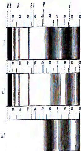
Fig. 24. Absorption spectrum of chlorophyll (after KÄRST, 1872). I, alcoholic extract of the green leaf (crude chlorophyll); II, spectrum of the blue-green benzene extract; III, spectrum of the yellow pigment. (From DEWEAR'S Smaller Practical Physiology .)
