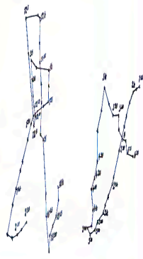
Fig. 16a. Projection curve of Phytomyza minor , after FRITSCHER (1869). \times 200 .
