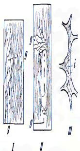
Fig. 100. Mode of growth of transplanted portion of beet. I, tangential section through the upper end of a portion of tissue inserted in the normal orientation. The limits of the tissue are indicated by the dotted lines gg. The longitudinal lines indicate vessels. II, a similar section of an inverted plug. The vascular bundles are developing almost entirely in the long axis. I and II about natural size. III, individual cells from the zones of fusion; a, intercellular spaces and thickened cell-walls. X about 50x. After VIGNON, 1891.
