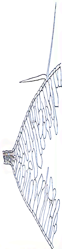
Fig. 95. Part of a transverse section through the middle-gall of Ullmannia dioica ; a part of the unaltered leaf is seen on the left-hand side. After KÜSTER (Pflanzl. Anatomie, Jena, 1904).
