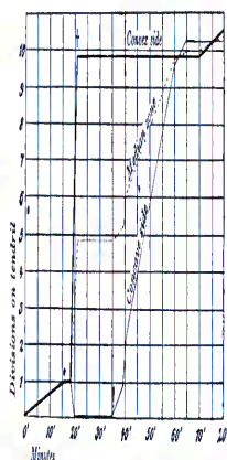
Fig. 154. Graphic representation of the growth of a tendril of Sida argentea . a , beginning of the stimulation; b , completion of the curvature; c , beginning of the readjustment.
