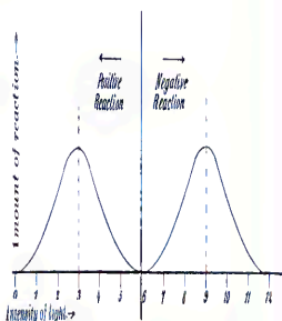
Fig. 146. Diagrammatic curve, to show the relation of heliotropic reaction to light intensity.
