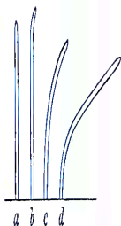
Fig. 149. Heliothetic curvature in Avena . After BOTTNER (from LIEBERMANN'S Practical Botany). a) not seen, a, at the commencement of the experiment; b, after 2½ hours; c, after 3½ hours; d, after 5½ hours.
