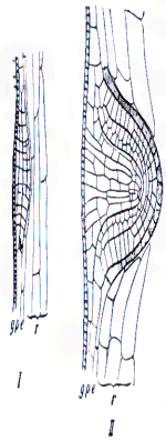
Fig. 81. Portion of a longitudinal section through the main axis of Rhodospira : a , apical cell; r , primary epidermis; r , cortex. After VAN DERZANDEN (Ann. sci. nat. 1901, ser. 7, vol. 8).
