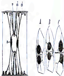
Fig. 58. Division of a cell of Spongova , a, daughter-cells; b, partition wall; c, chloroplast ( \times 190 ). (From the Bonn Textbook.)
