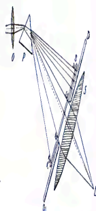
Fig. 26. Diagrammatic sketch of a spectroscop (after REINKE, Bot. Ztg. 1886, p. 1, fig. 2). O, projection lens; P, prism; SS, slit of \lambda = 50 to \lambda = 97 ; D, D', diaphragm for cutting off excessive rays; S, converging lens; L, position of the plate experimented on.
