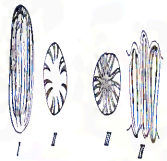
Fig. 125. Anthers of Lathium creditulum . I, isolated fibrous cell in the wet state. II, the same as seen from within. III, as seen from within. IV, as seen in section after drying. After STEINBRINCK (1898) \times 150 .
