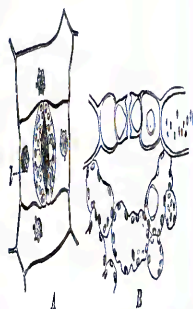
Fig. 7. Lower epidermis of Tradescantia virginica . A, from above; two guard-cells centrally placed; B, in section, showing below the guard-cells the respiratory cavity, on which the chloroplast-bearing paracytium abuts. \times 400 . (From the Bonn Yearbook.)
