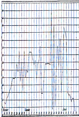
Fig. 86. Daily growth increments (in cm.) in the stem of Bambusa , measured at Balesberg from Nov. 13, 1895, to Jan. 10, 1896. After Kraus (ibid., Pl. 20)
