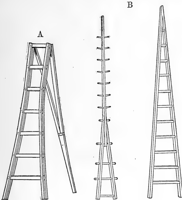
FIG. 4. Types of fruit ladders.
