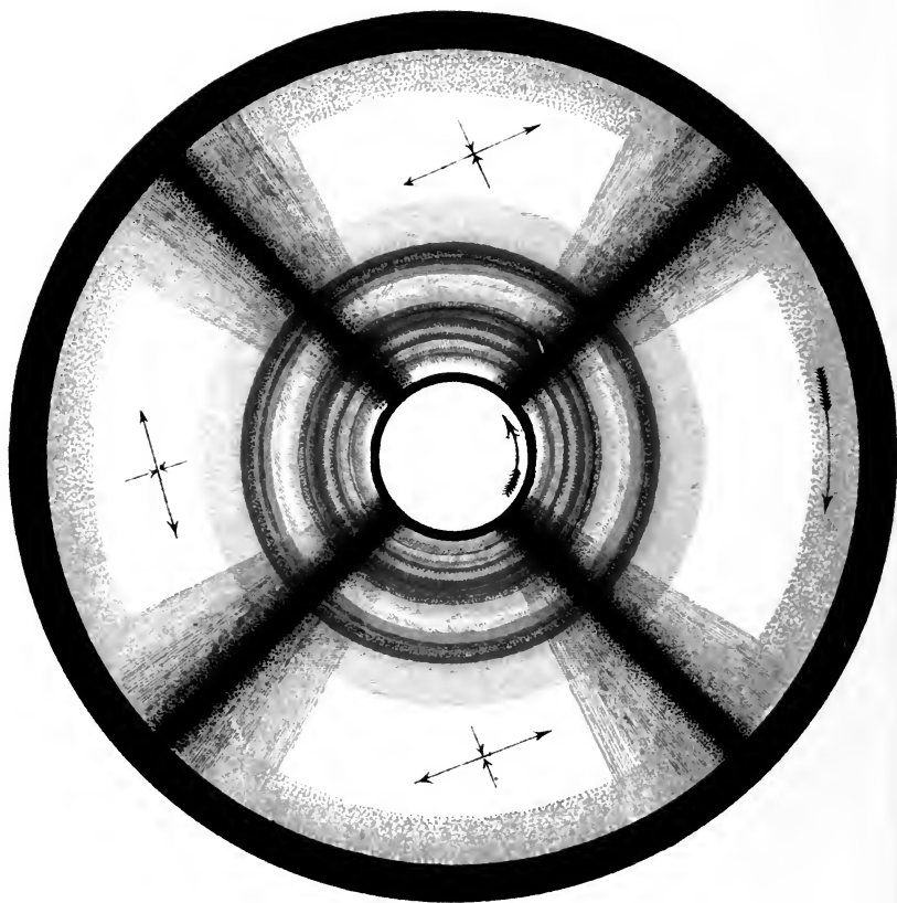
DIAGRAM SHEWING THE COLOURS EXHIBITED BY A PLATE OF GELATINE WHEN EXPOSED TO A TORSIONAL SHEAR.
