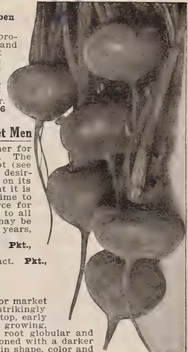
Crosby's Egyptian.
