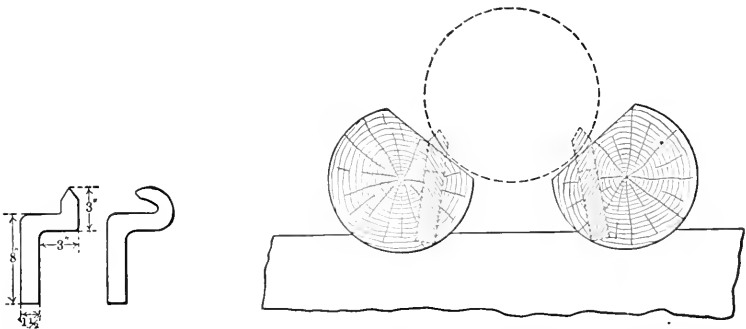
FIG. 94. — Two Common Forms of Goose-necks used for checking the Speed of Logs on Heavy Grades, and the Manner of placing them in the Slide Timbers.
