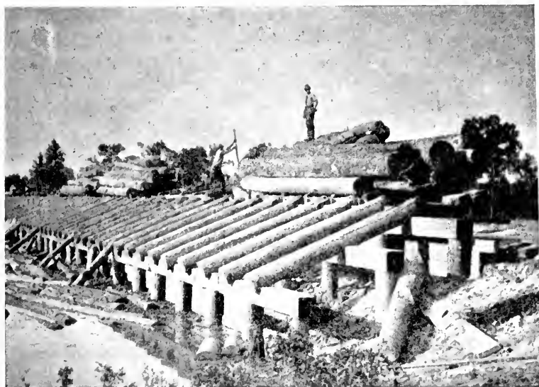
FIG. 130. — A Rollway at the Mill Pond. Texas.
