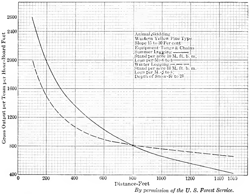
Fig. 36. — Graph showing the Influence on Skidding Output, Animal Logging, of Summer and Winter Conditions. Inland Empire.
