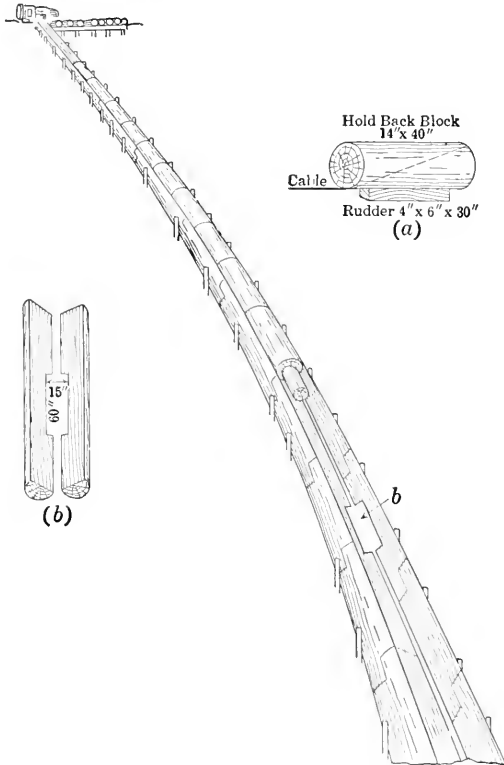
FIG. 95. — A Snubbing Device for lowering Logs down a Chute.
