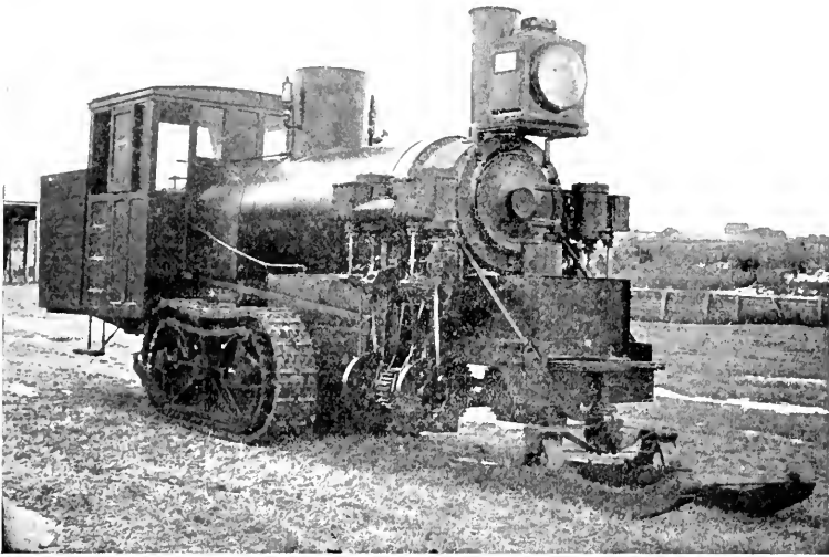
Fig. 50. — A Lombard Steam Log Hauler.
