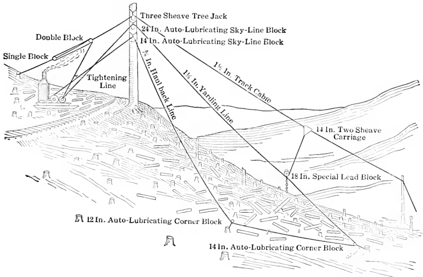
FIG. 70. — The North Bend System of Overhead Logging.
