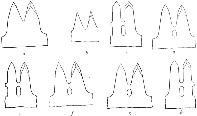
FIG. 10. — The Forms of Bevel used on Cross-cut Saws. a . Diamond point bevel, easy to maintain, and the point holds well. b . Bevel for a tooth where there are no rakers, the teeth cleaning out the sawdust. c . Bevel for knots and frozen timber where strength is needed in the extreme point — not adapted for fast-sawing. d . Round point for fast, smooth sawing, in knotty timber. e . Bevel for fast, smooth sawing — teeth strong. f . Flat, thin bevel for soft wood and fast sawing — point is not as strong as that shown in e . g . Bevel adapted for general work. h . Bevel adapted for general work.
