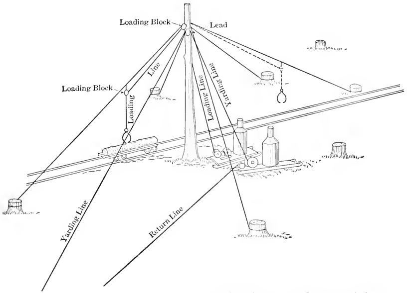
FIG. 128. — A Single Guy-line Loading System. Pacific Coast Forests.
