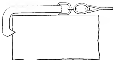
FIG. 93. — An "L" Hook used for attaching the Tow Line to the Turn of Logs.
