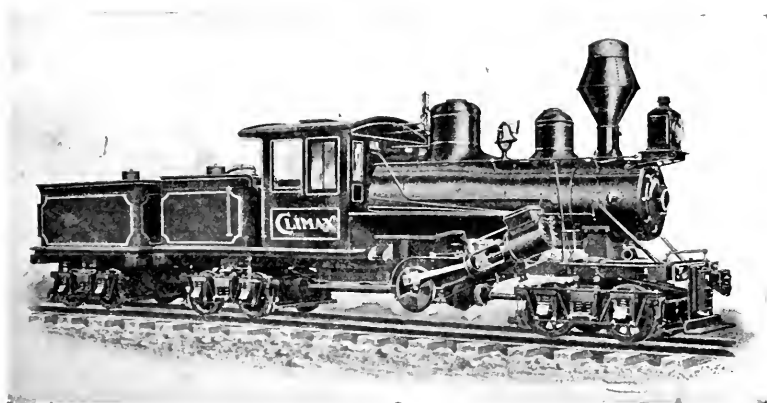
FIG. 114. — A Climax Geared Locomotive.
