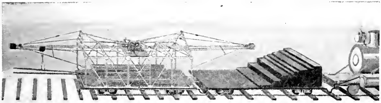
FIG. 110. — The Norby Track-Laying and Lifting Device..
