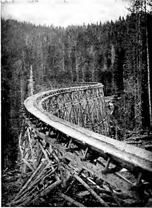
FIG. 159. — A V-flume for transporting Mining Stulls. Montana.
