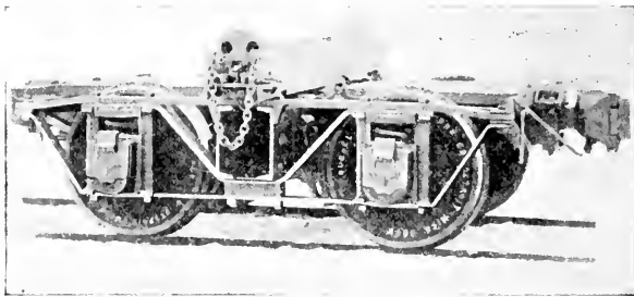
FIG. 120. — A Log Truck, Western Type.
