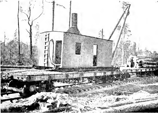
FIG. 123. — The Rapid Log Loader.
