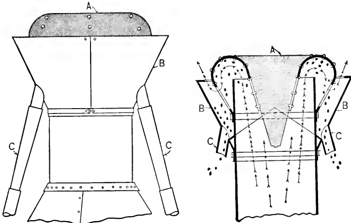
FIG. 117. — The Sequoia Spark Arrester.
