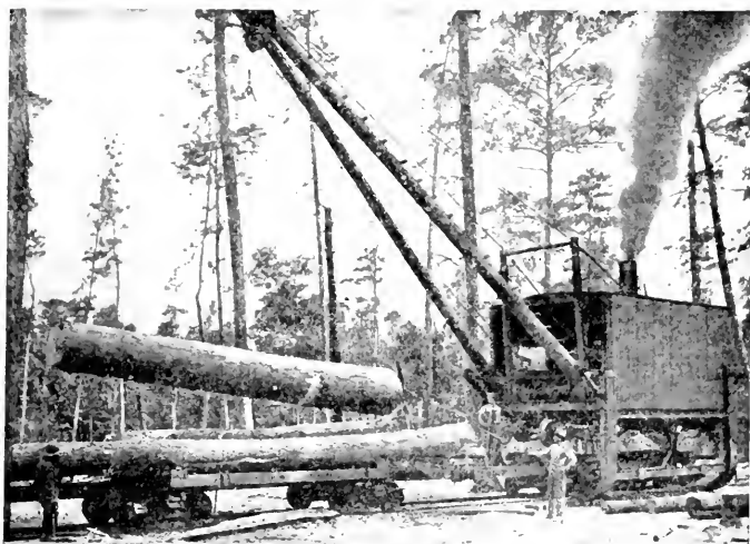
FIG. 125. — The McGiffert Log Loader.
