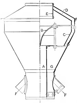
Fig. 118. — The Radley-Hunter Spark Arrester.
