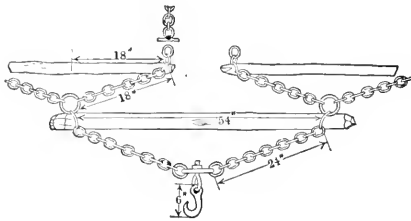
FIG. 31. — A Common Type of Spreader used in skidding on Slopes and Rough Ground.
