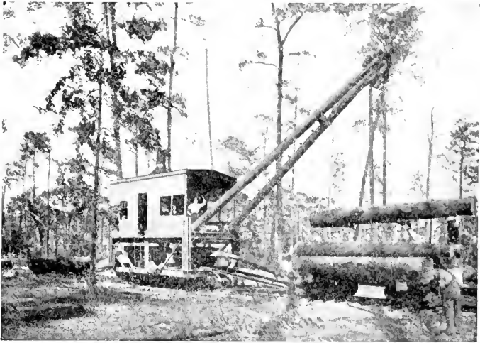
FIG. 124. — The Decker Log Loader.
