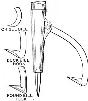
FIG. 16. — A Socket Peavey.
