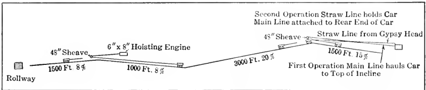
FIG. 112. — An Incline System used to transport Timber across Two Ridges.
