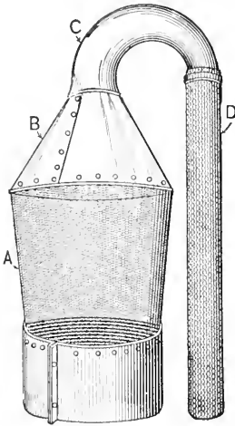
FIG. 80. — The Boomerang Spark Arrester.
