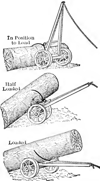
FIG. 52. — The Method of loading Logs on a Bumper.
