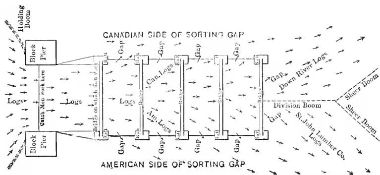
FIG. 144. — A Sorting Gap on the St. John's River near Fredericton. New Brunswick.
