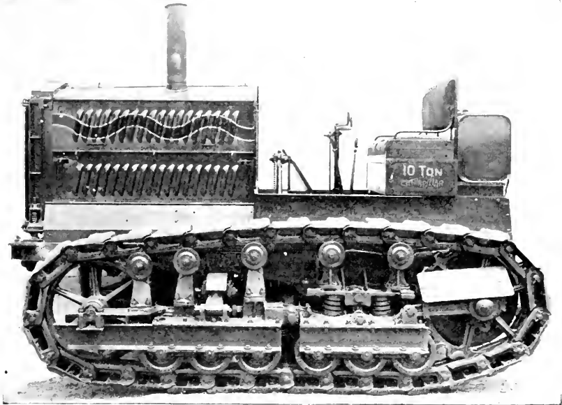
FIG. 59. — A Holt 10-ton Caterpillar Tractor showing the General Features of one of the Traction Members.
