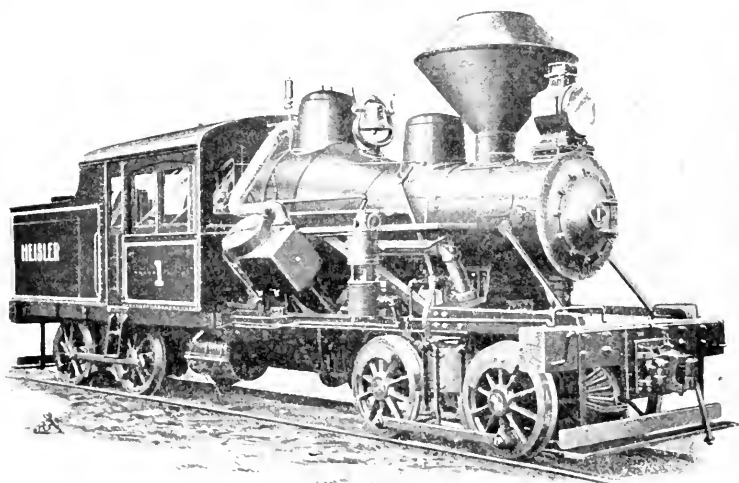
FIG. 115. — A Heisler Geared Locomotive.
