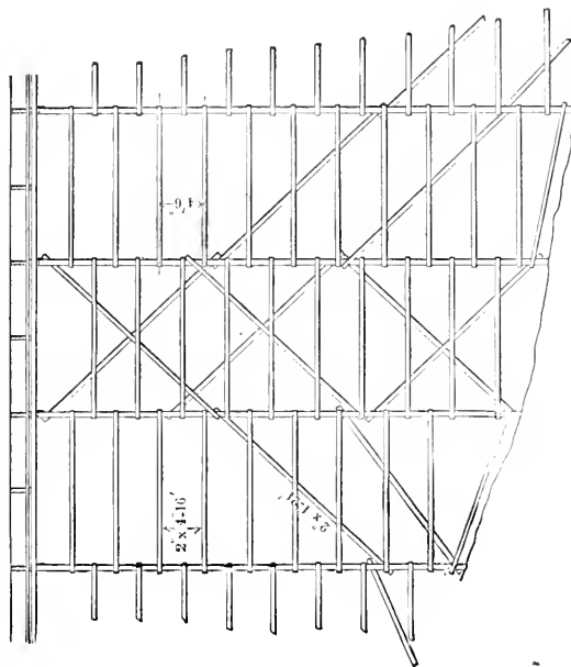
VIEW SHOWING METHOD OF "X" BRACING TO BE USED EVERY 10TH SPAN
