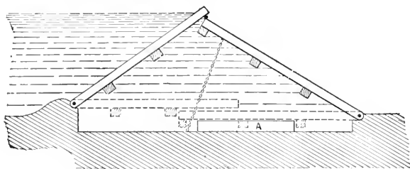
FIG. 135. — The Bear-trap Sluice Gate.
