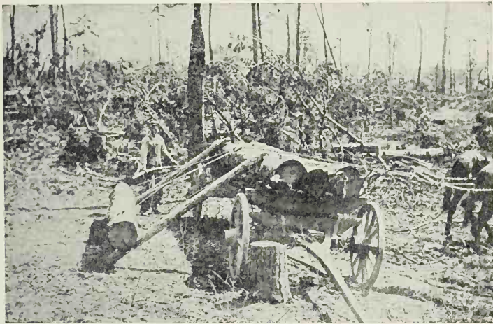
FIG. 57. — Loading a Log Wagon by means of the Crosshaul. The teamster is doing his own loading. Missouri.
