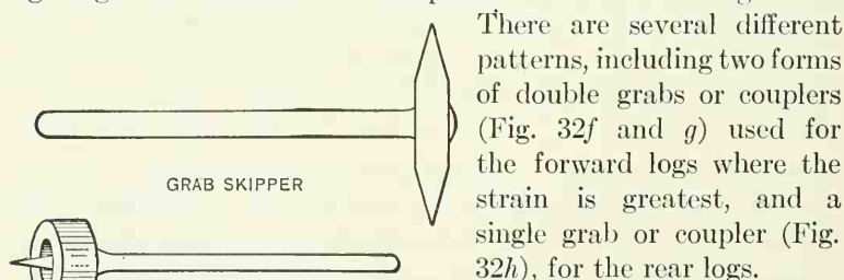
FIG. 34. — A Type of Grab Skipper and a Grab Maul used on a West Virginia Logging Operation.
