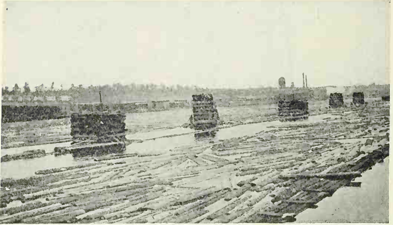
FIG. 142. — Piers placed in a River to hold Storage Booms. Minnesota.
