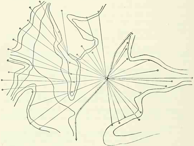
FIG. 68. — A Logging Chance showing the Use of an Overhead Cableway System in bringing Timber over a Ridge by relaying
