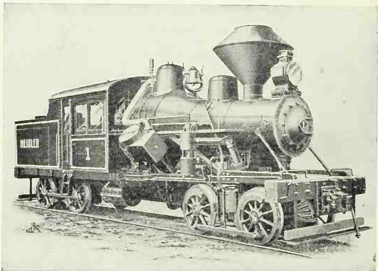
FIG. 115. — A Heisler Geared Locomotive.
