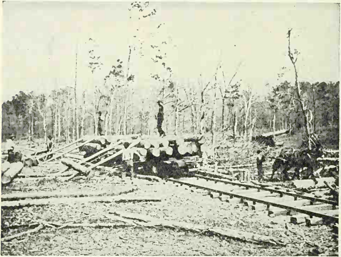
FIG. 121. — Loading Log Cars with a Crosshaul. Missouri.
