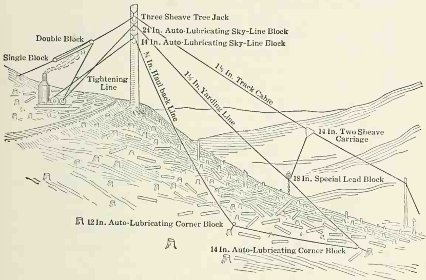
Fig. 70. — The North Bend System of Overhead Logging.
