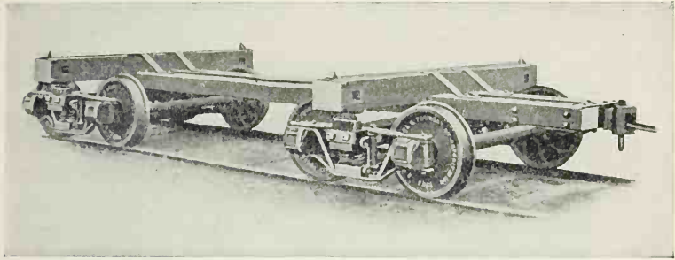
FIG. 119. — A Skeleton Log Car. A type common in the southern yellow pine forests.
