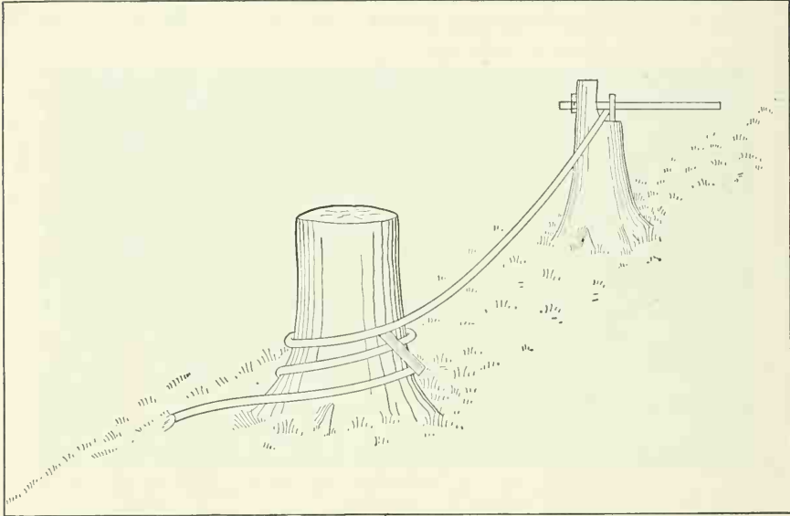
FIG. 48. — A Snubbing Device for controlling the speed of Loaded Sleds on Steep Grades. The free end of the rope in the foreground is attached to the sled.
