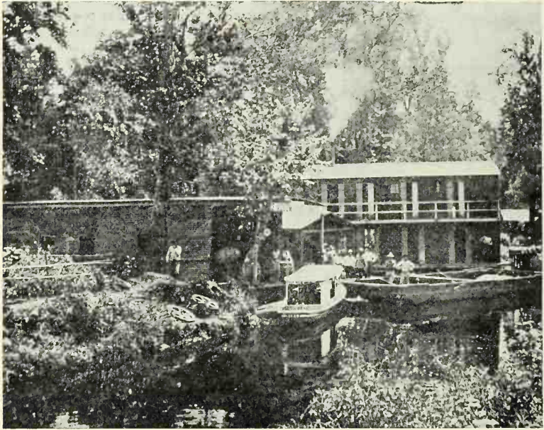
FIG. 6. — A Floating Camp on a Cypress Operation. The dining room and office are on the ground floor and the sleeping quarters are in the upper story. The building on the left is the camp store. Louisiana.
