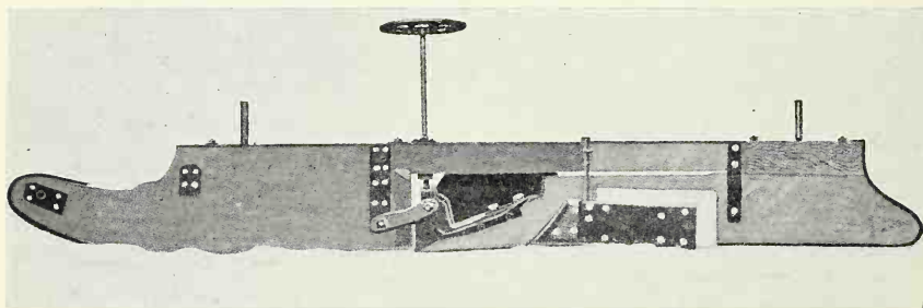
FIG. 46. — The Badger Rut Cutter (side view).
