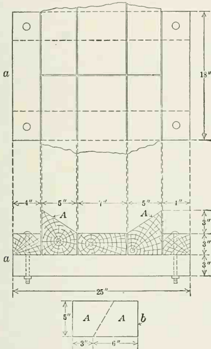
FIG. 90. — The Sykes Trailing Log Slide.
