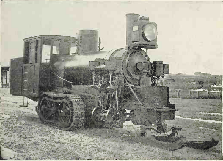
FIG. 50. — A Lombard Steam Log Hauler.
