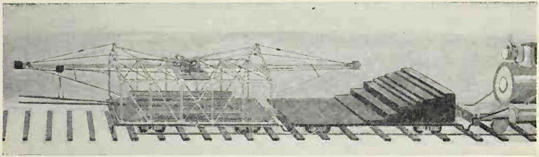
FIG. 110. — The Norby Track-Laying and Lifting Device..
