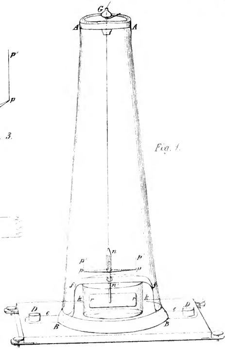
Prof. Draper's Improved Torsion Balance.
