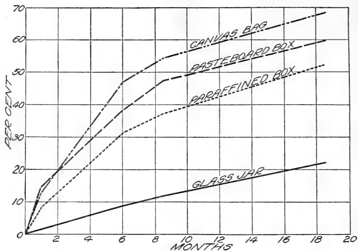
FIG. 7.—Loss of nicotine from free nicotine-kieselguhr dust
