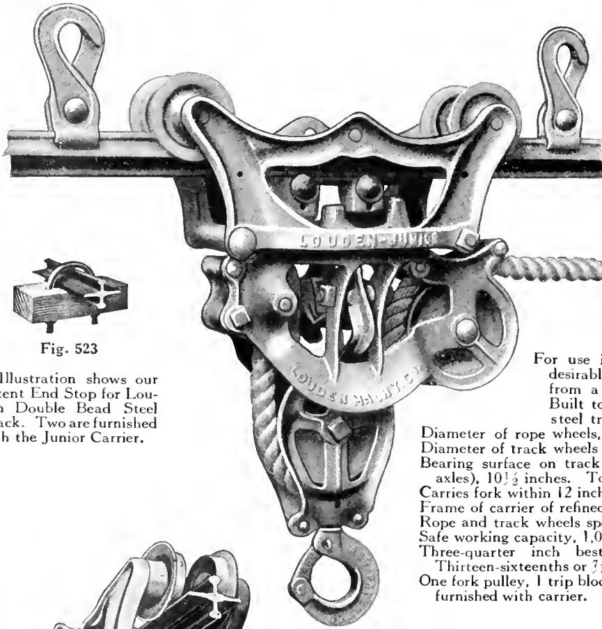
Trip Block Furnished as Part of Carrier
