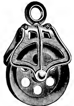
Fig. 495 (Password) Fig. 495. Draft Pulley. Malleable frame, swivel eye, 6-inch diameter sheave. Sheave made of special quality gray iron. Weight, 5½ pounds.
