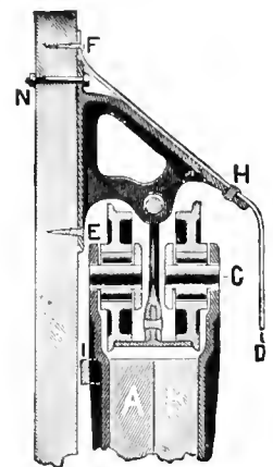
Fig. 453 Sectional View
