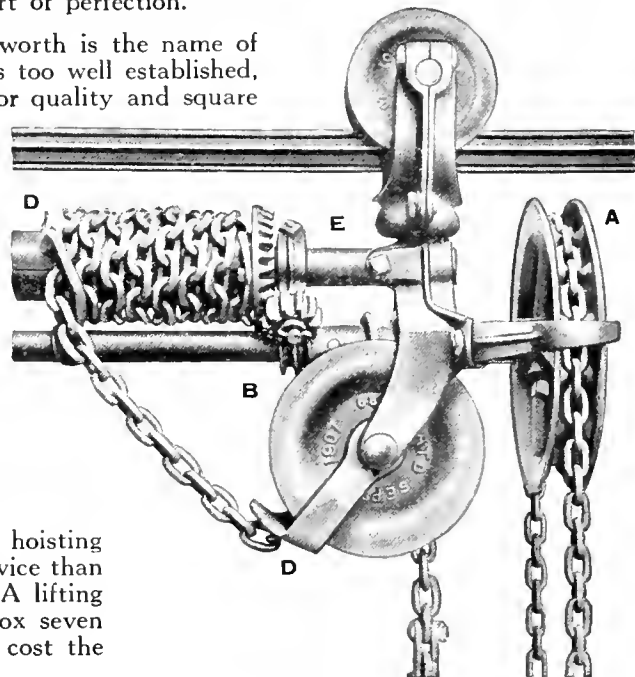
Fig. 881. The Emancipator Hoisting Gear.
