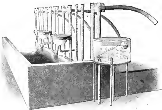
"Ghost View" of Governing Tank and Bowls. The water in the tank and bowls is kept at the same level by means of the ball float.
