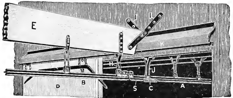
Fig. 859. Junior. (Gait). Patented Nov. 13, 1909
