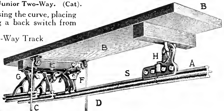
Fig. 795. Three-Way Switch. (Caboose).
