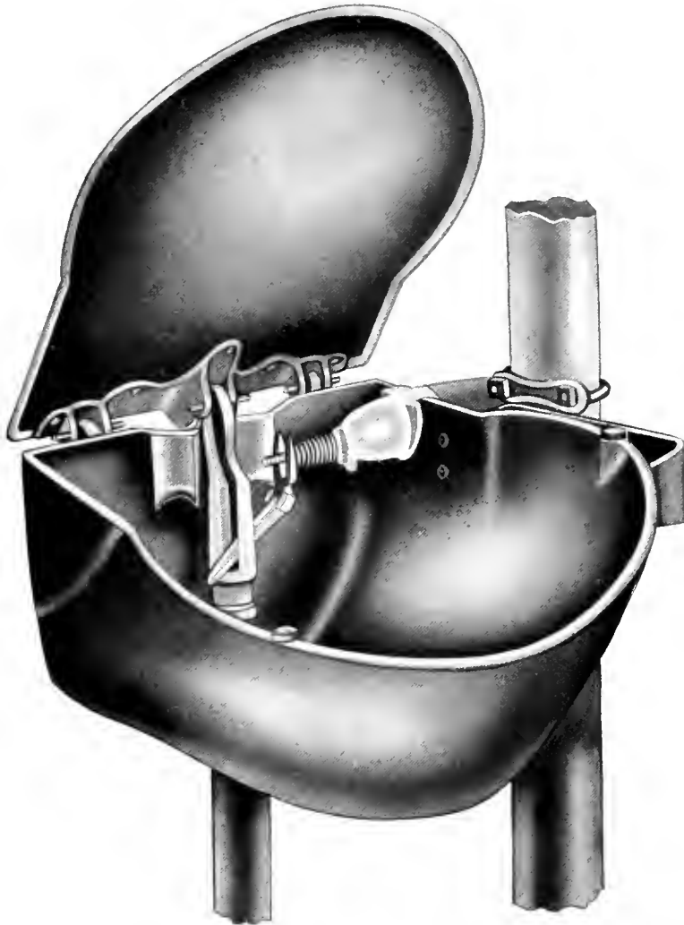
Fig. 1294—Inside View showing Simple Mechanism of Bowl. It's always in "working order."
