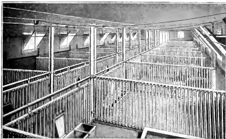
Hog House on Homewood Farms, Moline, Ill.—Louden Equipped hog houses in this country. It is fitted throughout with the Louden Tubular Steel Hog Pens. It is kept so clean and is so well ventilated that it is entirely free from the disagreeable odor common to hog pens.
