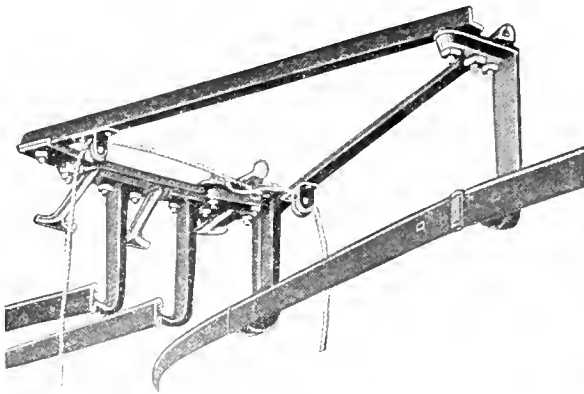
Fig. 1296 Three-Way Switch for Combination Track
