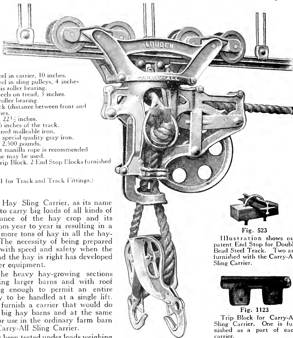
Fig. 1103 (Heavy) Patent Pending
