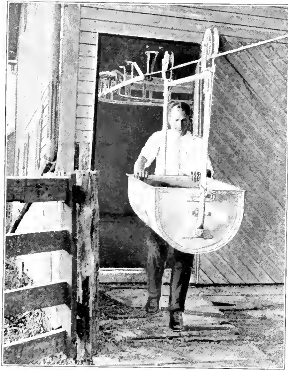
Fig. 1287—Using the Louden Self-Acting Carrier on the Louden Combination Steel and Rod Track
