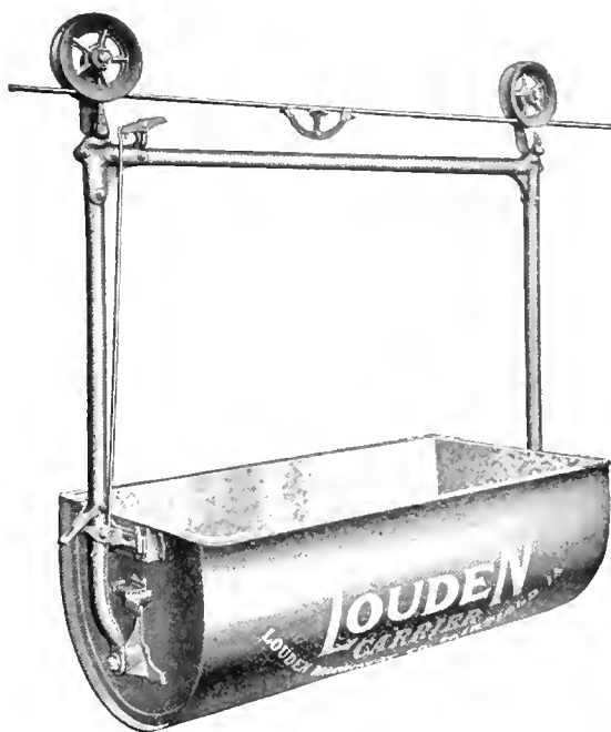
Fig. 721. (Hymn). Patented Oct. 6, 1908.
