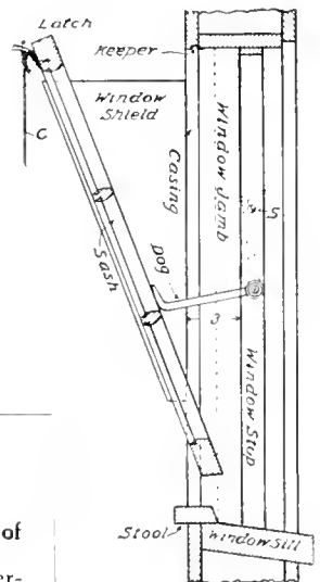
Fig. 989 Cross Section
