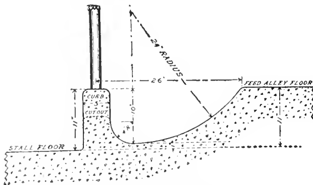
Fig. 1001 Louden Low Cement Manger, with Raised Feed Alley Floor
