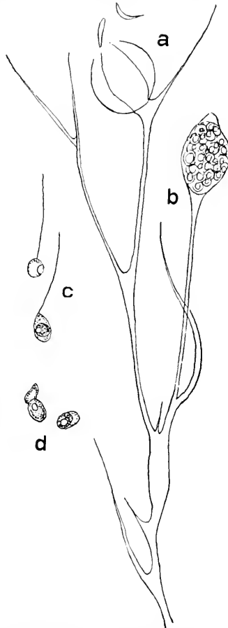
FIG. 33.— Nowakowskiella degans (Nowak.) Schröter. (a) Terminal sporangium on branching mycelium; secondary sporangium formed by proliferation within the primary; lids of both fallen away. (b) Swarmsporangium containing spores. (c) Swarmspores. (d) Amoeboid zoospores. (After Nowakowski 1876.)
