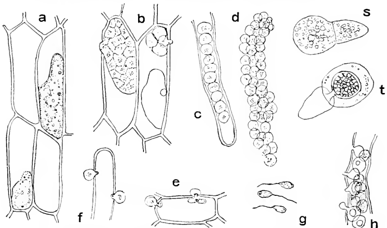
FIG. 5.— Rhizomyxa hypogaea Borzi. (a) Young thalli in cortical cells of Stellaria media . (b) Formation of sporangia. (c, d) Sori of sporangia, that at (c) in a root hair. (e, f) Zoospores infecting host cells. (g) Swarmspores. (h) Germinating sporangia with exit tubes. (s) Thallus divided by septum to form oogonium and antheridium. (t) After fertilization showing oospore in oogonium. (After Borzi 1884.)
