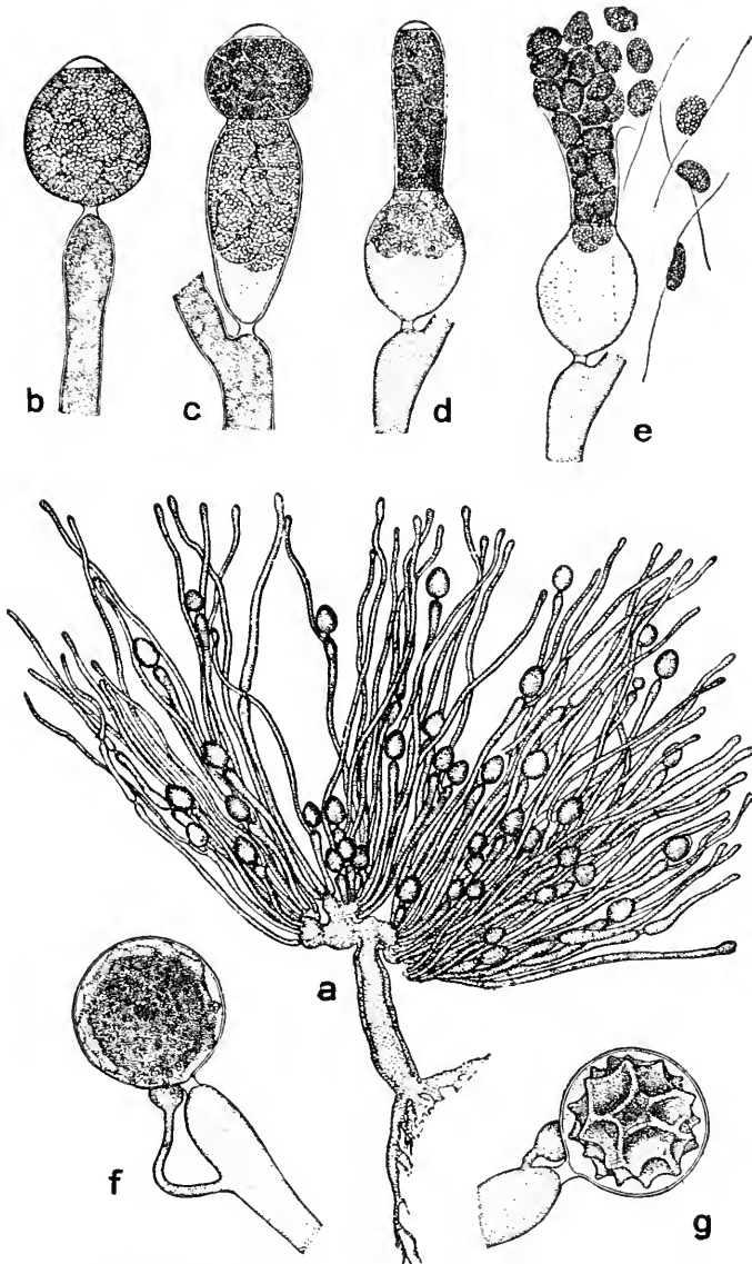
FIG. 68.— Rhipidium americanum Thaxter. (a) Typical plant, the branches showing occasional segmentation. (b-e) Sporangium with papilla of dehiscence extruding swarmspores into a thin-walled vesicle which finally ruptures freeing biciliate swarmspores. (f) Oogonium in which the exospore is being formed by the periplasm. (g) Mature oospore. (After Thaxter 1896.)
