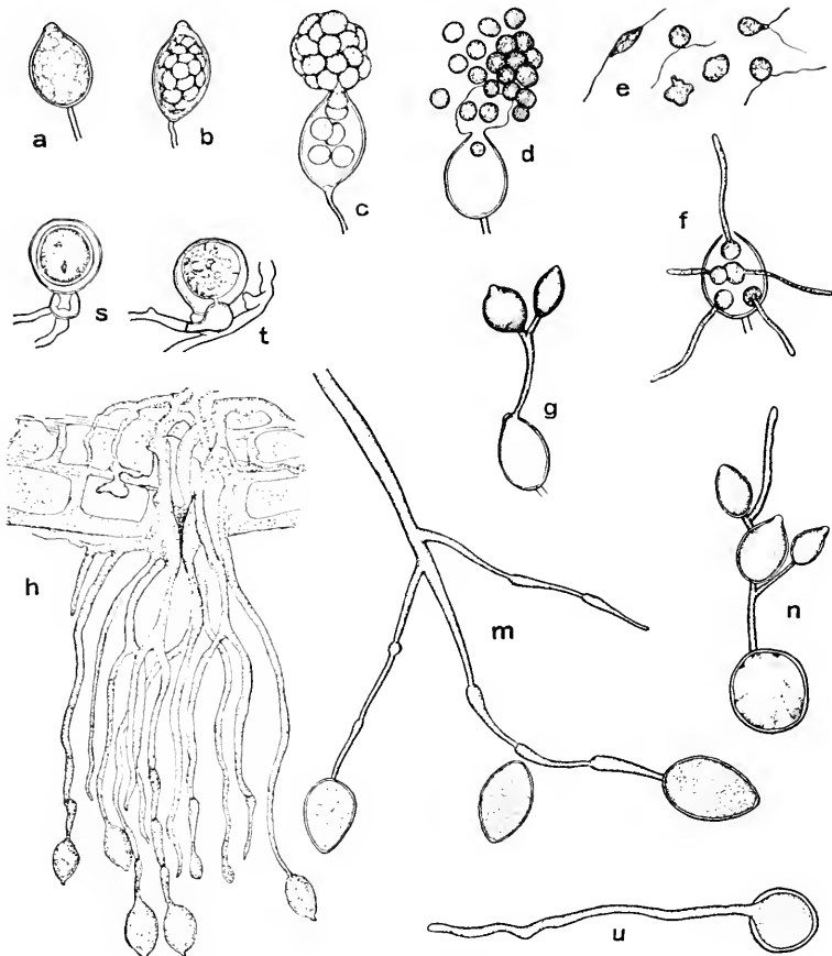
FIG. 72.— Phytophthora spp. (a-e) Germination of sporangium by swarmspores, the spores passing first into a vesicle. (f) Sporangiospores which failed to escape germinating by germ tubes in the sporangium. (g) Secondary sporangia developed at tip of germ tube of primary sporangium. (h) Sporangiophores of Ph. phaseoli arising from a stomate of lima bean. (m) Sporangiophore of Ph. infestans . (n) Oospore germinating by a germ tube on which sporangia then form. (s) Oogonium, basal antheridium, and oospore in Ph. erythrocephala . (t) Oogonium, lateral antheridium, and oospore in Ph. cactorum . (u) Germination of oospore by simple germ tube. (h, after Thaxter 1889; m, after Schwarze 1917; others after Rosenbaum 1917.)
