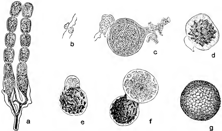
FIG. 69.—(a) Albugo portulacae (DC.) Kuntze, showing sporangiophores and chains of sporangia. (b-f) A. candida (Pers.) Kuntze. (b) Swarmspores. (c) Young oogonium and antheridium. (d) Mature oospore in oogonium. (e-f) Germinating oospore. (g) A. tragopogonis (DC.) Gray; mature oospore. (g, after Schwarze 1917; others after de Bary 1887.)
