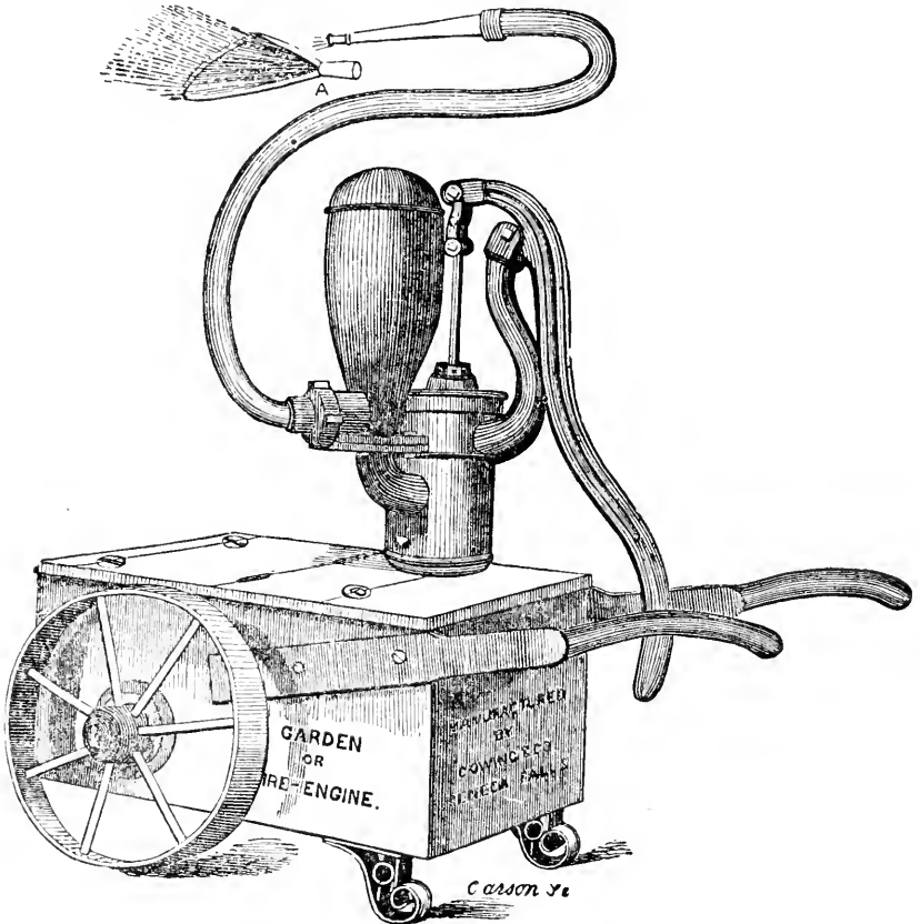
47. GARDEN ENGINE, WITH WATER DIFFUSER.
