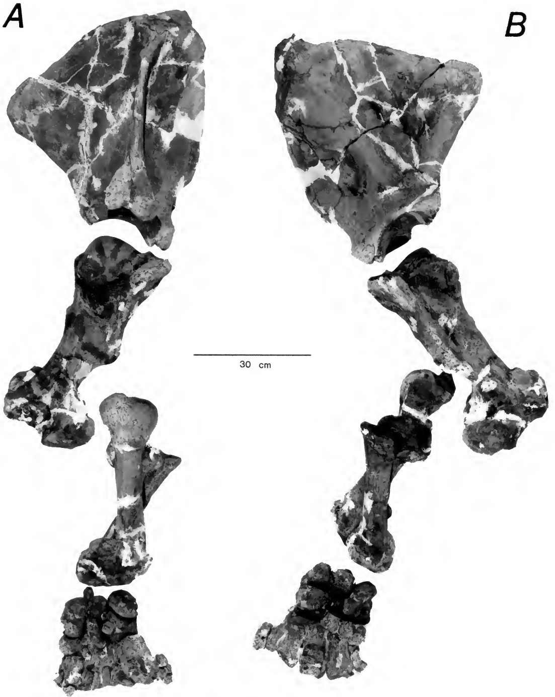
FIG. 45. Uintatherium anceps , articulated right forelimb of the partial skeleton. PM 55423, collected by J. J. Flynn and his field crew. A and B show approximately opposite sides of each set of elements laid out separated, except the manus, which is still held in the position in which it was found by a thin layer of matrix (FMNH neg. nos. GEO 85930.5 and 85930.7).
