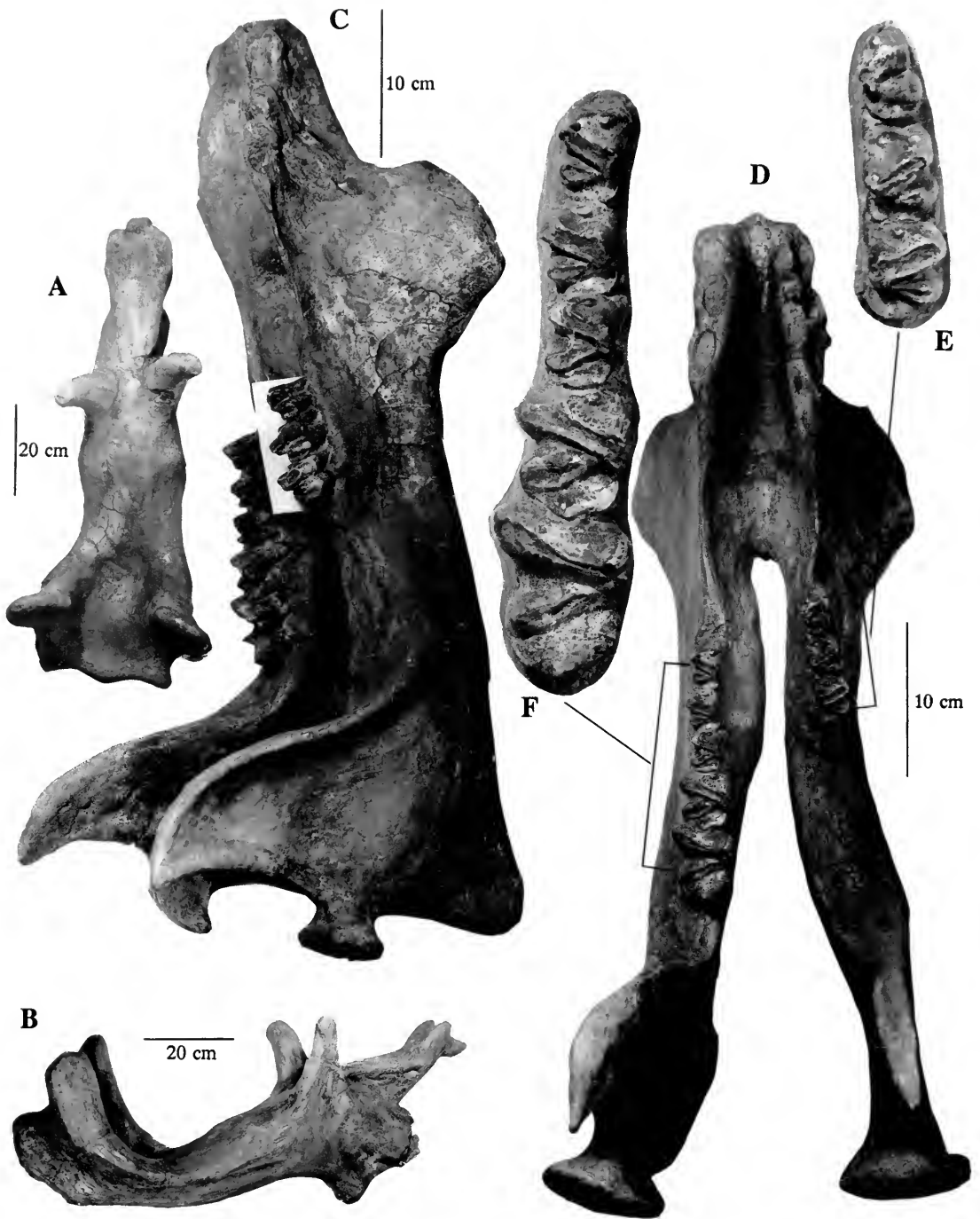
FIG. 60. Partial skull (A and B, dorsal and right lateral views) and mandible (C and D, right lateral and occlusal views) of Tinoceras annectens Marsh (= Tetheopsis speirianus (Osborn) = E. cornutus ), in the Yale University collection, YPM VP 11043. The skull is considerably restored, but its dorsal surface is largely preserved. In the mandible there are three incisor alveoli on each side of the symphysis, and the inframandibular processes are prominent. The left cheek-tooth series, which preserves p3-m3, and the right series with p2-p4, are shown in occlusal views in E and F (FMNH neg. nos. GEO 82428-31).
