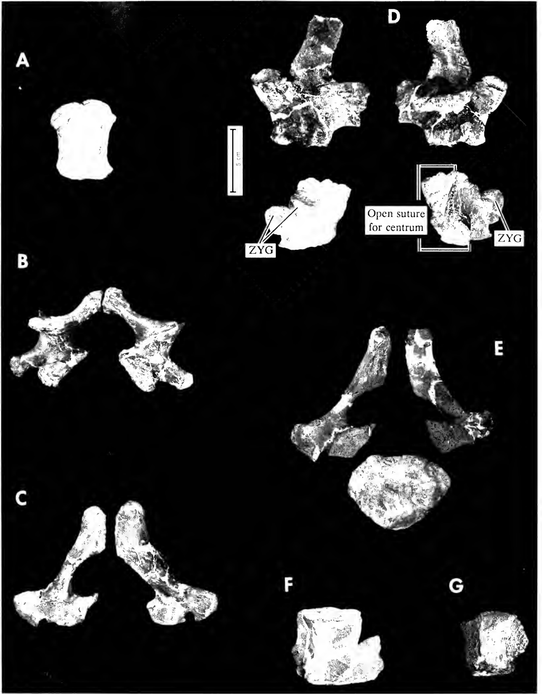
FIG. 41. Uintatherium anceps juvenile, probably newborn, PVI 3896. A , Second sternal element shown in presumed ventral view. B–G , A series of the vertebrae exhibiting their early development, before fusion of arch elements and centrum. In most cases the positions indicated are approximate. B , Posterior views of arches of the 3rd cervical on left and 4th cervical on right, posed as though belonging to a single vertebra. C , Arches of two different anterior thoracic vertebrae seen in anterior view, again posed as a pair. Both have facets for rib articulation that lack epiphyseal caps. D , top left , dorsolateral view of a left neural arch (anterior end to right), and top right , the reverse (ventromedial)
