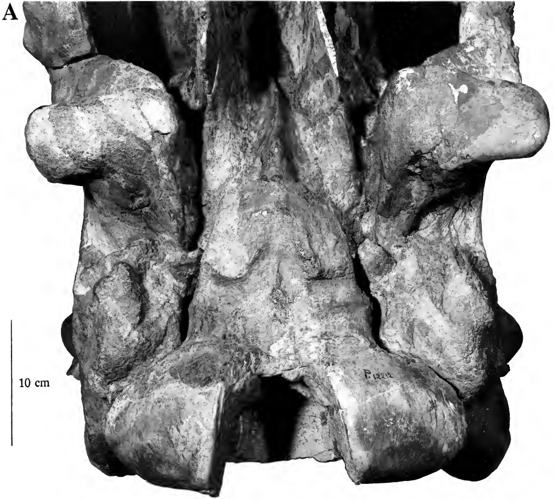
FIG. 29. Basicranial region of FMNH P 12170 (= P12212 in error), the Field Museum's fine specimen of Eobasileus cornutus (called E. uintensis by Osborn in 1929, a nomen nudum) is shown in A . B provides the key to its features (FMNH neg. no. GEO 85914).
