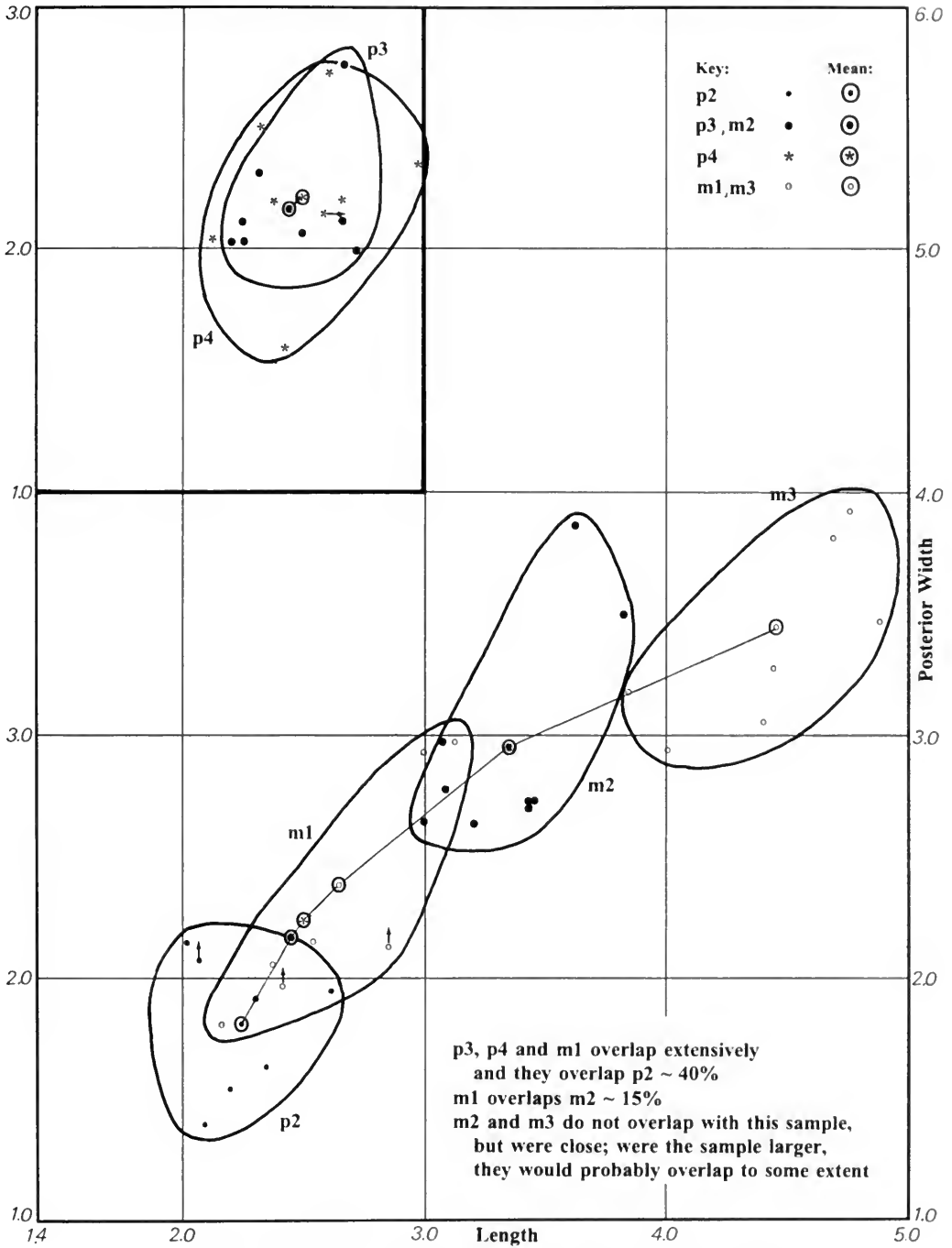
FIG. 65. Bivariate graph of lower cheek teeth of E. cornutus . Measurements are in cm.
