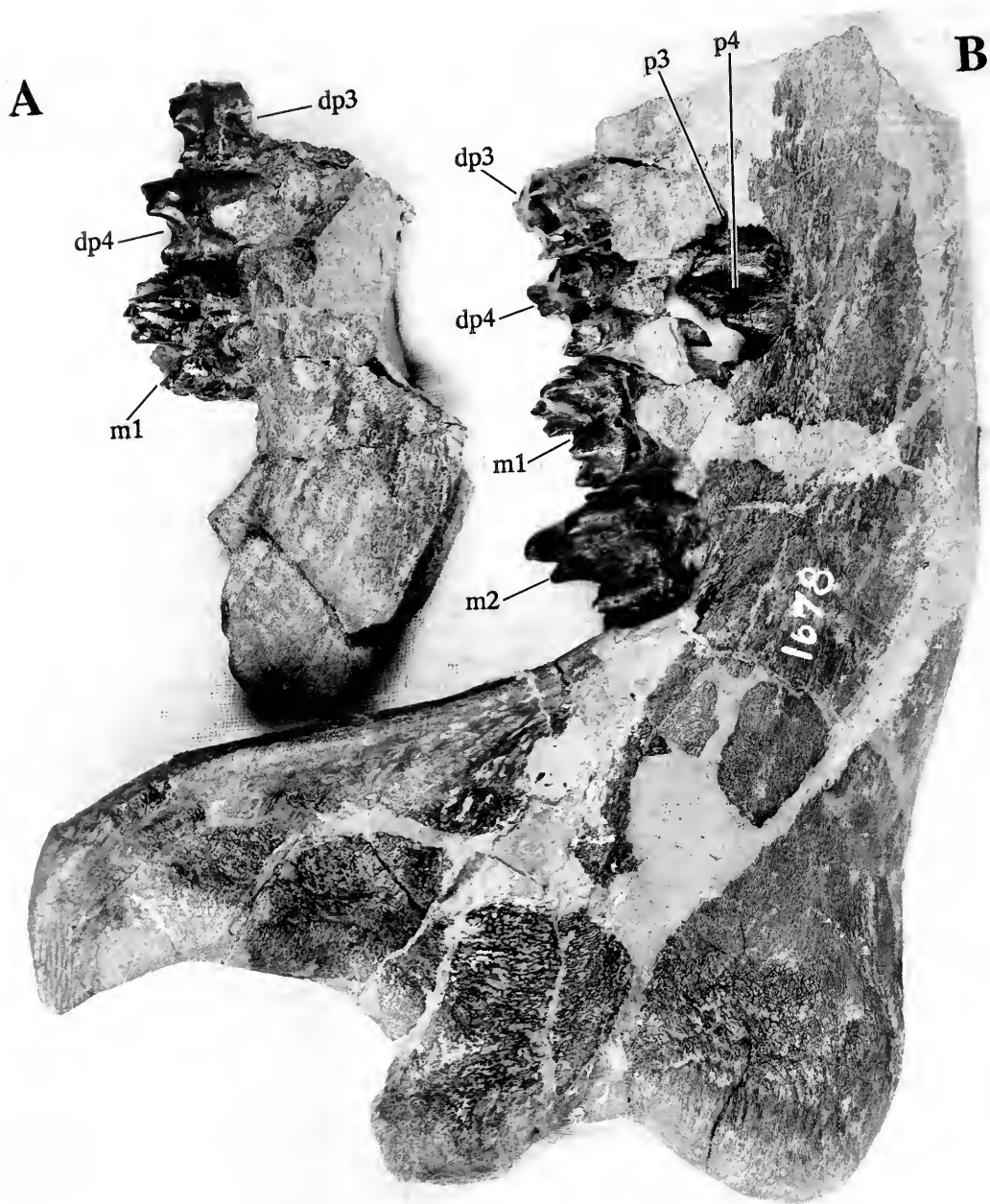
FIG. 31. U. anceps , AMNH 1678, a pair of juvenile jaws and dentitions consisting of the posterior two-thirds of the right mandibular ramus (B and C) including the coronoid, condylar, and angular processes, and (A and D) a fragment of the left ramus. Preserved teeth are L and R dp3-4, m1; R p3-4, m2. Also present are L m2 alveoli, and a portion of the wall of the crypt for m3. This is the specimen that Wheeler (1961, p. 43 and Pl. 13) referred to as being the only example of a juvenile among the terminal North American uintatheres. I show it at a better scale with more detail (FMNH neg. nos. GEO 82498 (A, B) and 82499 (C, D)).
