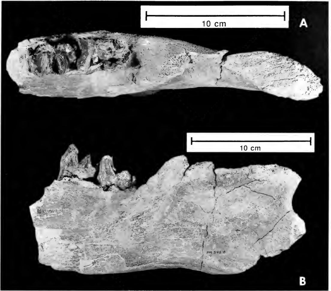
FIG. 33. PM 54818, part of the left jaw of a subadult Uintatherium anceps with M2-3 shown in dorsal (occlusal) view (A) and left lateral view (B). This is one of several subadult and juvenile specimens in the FMNH collection (FMNH neg. nos. GEO 85688 and 85708).
