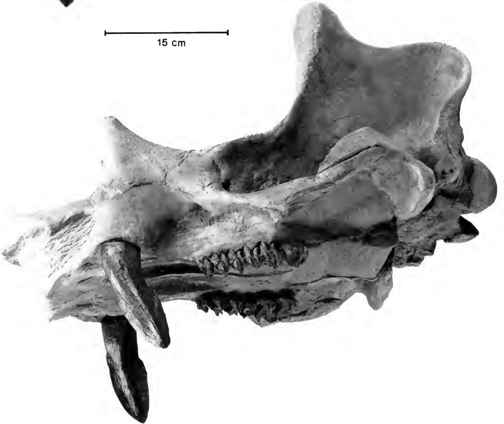
The beautifully preserved Funderburk skull of Uintatherium anceps , PM 53933 (FMNH neg. nos. GEO 85354 and 85355).
