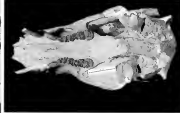
FIG. 71. Comparisons of upper cheek teeth of rhinoceroses (A–C) with those of U. anceps (D). A , Diceros bicornis , FMNH 85429; B , Ceratotherium simum cottoni , FMNH 29174; C Rhinoceros unicornis , FMNH 57639 (FMNH neg. nos. GEO 85970.1 and .3 (A); 85971.3 and ?? (B); 85970.8 and ?? (C); 85689 and 85?? (D)).
