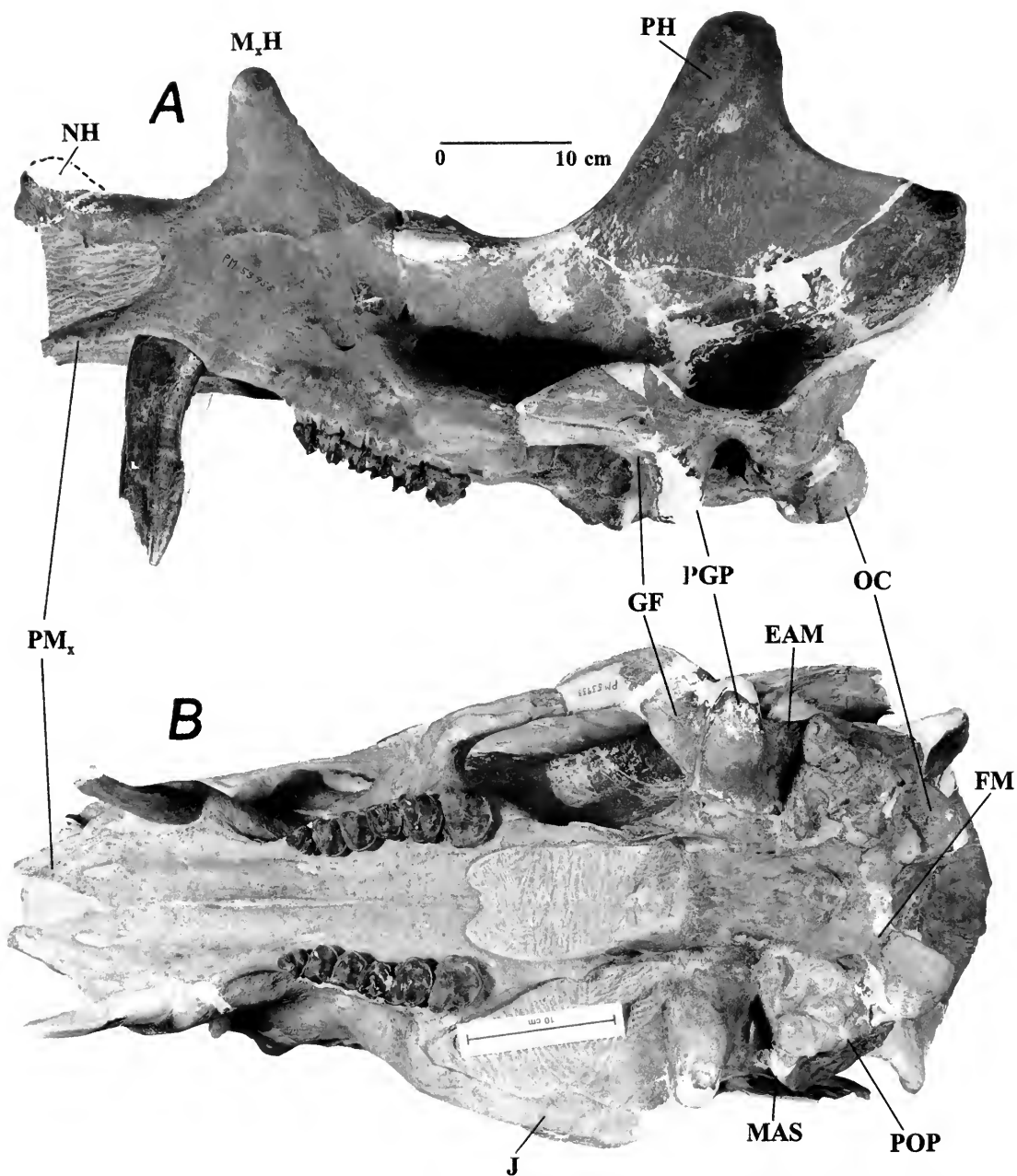
FIG. 5. A, Left lateral, B, ventral, C, dorsal, and D, inverted posterior views of the most complete adult Uimatherium anceps skull in the Field Museum's Washakie collection, the well-preserved Funderburk skull, PM 53933. The skull is that of a young adult male that is lacking only a minor bit here and there and most of its right canine tusk. Its cheek teeth are nearly unworn except for the M1s, on which the enamel of the lophs is breached, but the greater part of the structure of each loph remains. The relatively short horns and low parietal-occipital crests are further testimony to its young age state. It was discovered by the late Tom Funderburk, collected in 1984, and donated to the Museum in 1989. Abbreviations are identified in the captions to Figures 8 and 9, and others as needed. Scale for C is the same as for A and B (FMNH neg. nos. GEO 85689 (A), 85690 (B), 85799.1 (C), and 85799.2 (D)).
