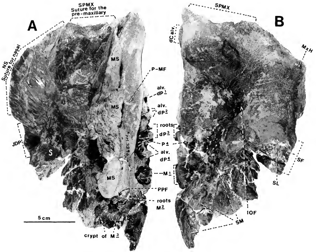
FIG. 9. Medial (A) and lateral (B) views of the same left maxillary as in Figure 8, PM 3896, showing the considerable depth of the skull in this region, the very immature maxillary horn bud, the extensive sutures for the nasal and premaxillary bones, as well as the near-midline suture of the palate. By comparing this "near-newborn" maxillary with the other juvenile and young adults, I estimate the skull length at about 40 to 45 cm. Associated with this specimen are many postcranial elements, including a scapula, an ilium, and vertebral elements (Figs. 46, 49 and 41, 42). The teeth, alveoli, and other tooth features are labeled using standard dental abbreviations. Other abbreviations are: J-DP = juvenile-dorsal pit (of uncertain significance), IOF = infraorbital foramen, MS = midline palatal suture, MxH = maxillary horn bud, NP = nasal passage, P-MF = palato-maxillary foramen, S = sinus cavity, SF = suture for frontal, SL = suture for lacrimal, SM = suture for malar, SN = suture for nasal, SPMx = suture for premaxillary (groove) (FMNH neg. nos. GEO 85779 and 85780).
