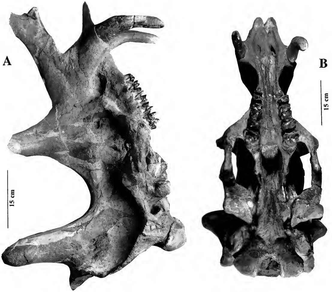
FIG. 55. Eobasileus cornutus from the Uinta Basin, P 12710. This is the only complete skull of this taxon in the FMNH collection. It was collected in 1910 by J. B. Abbott, chief assistant to E. S. Riggs, and is the most complete and well-preserved specimen of the species. It is shown in right lateral (A) and ventral (B) views. In C, the palate and cheek teeth are shown enlarged. The specimen has recently been installed in the new hall of fossil vertebrates (FMNH neg. nos. GEO 85710–11).
