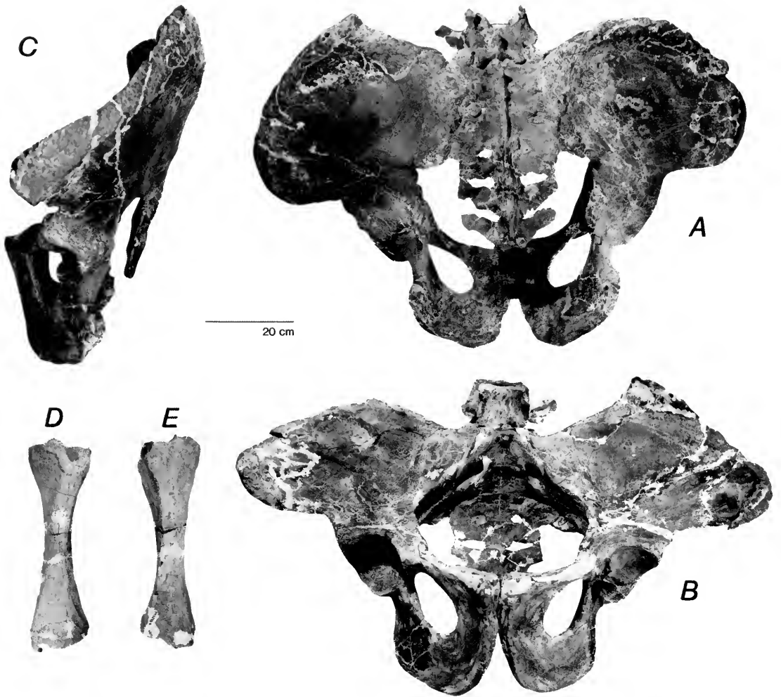
FIG. 50. Untatherium anceps , articulated pelvis with the last lumbar, vertebra, sacrum, and first three caudal vertebrae in place; PM 3894. It is shown in dorsal (A), ventral (B), and left lateral (C) views. In D and E, anterior and posterior views of a tibia, PM 38782, are shown (FMNH neg. nos. GEO 82120-2 and 86086-7).
