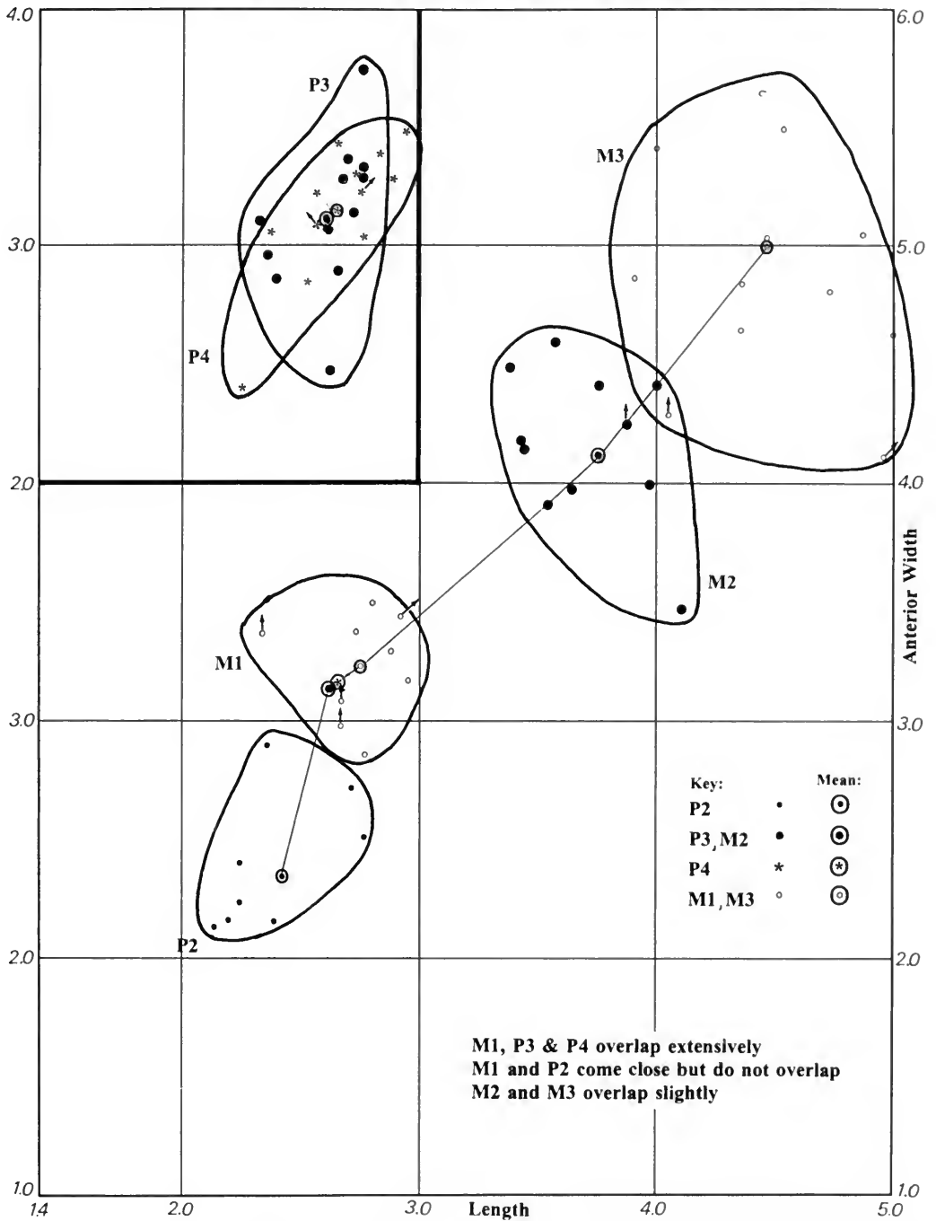
FIG. 61. Graph showing bivariate plots, length \times anterior width, for the upper cheek teeth of Eobasiliscus cornutus . Measurements are in cm.
