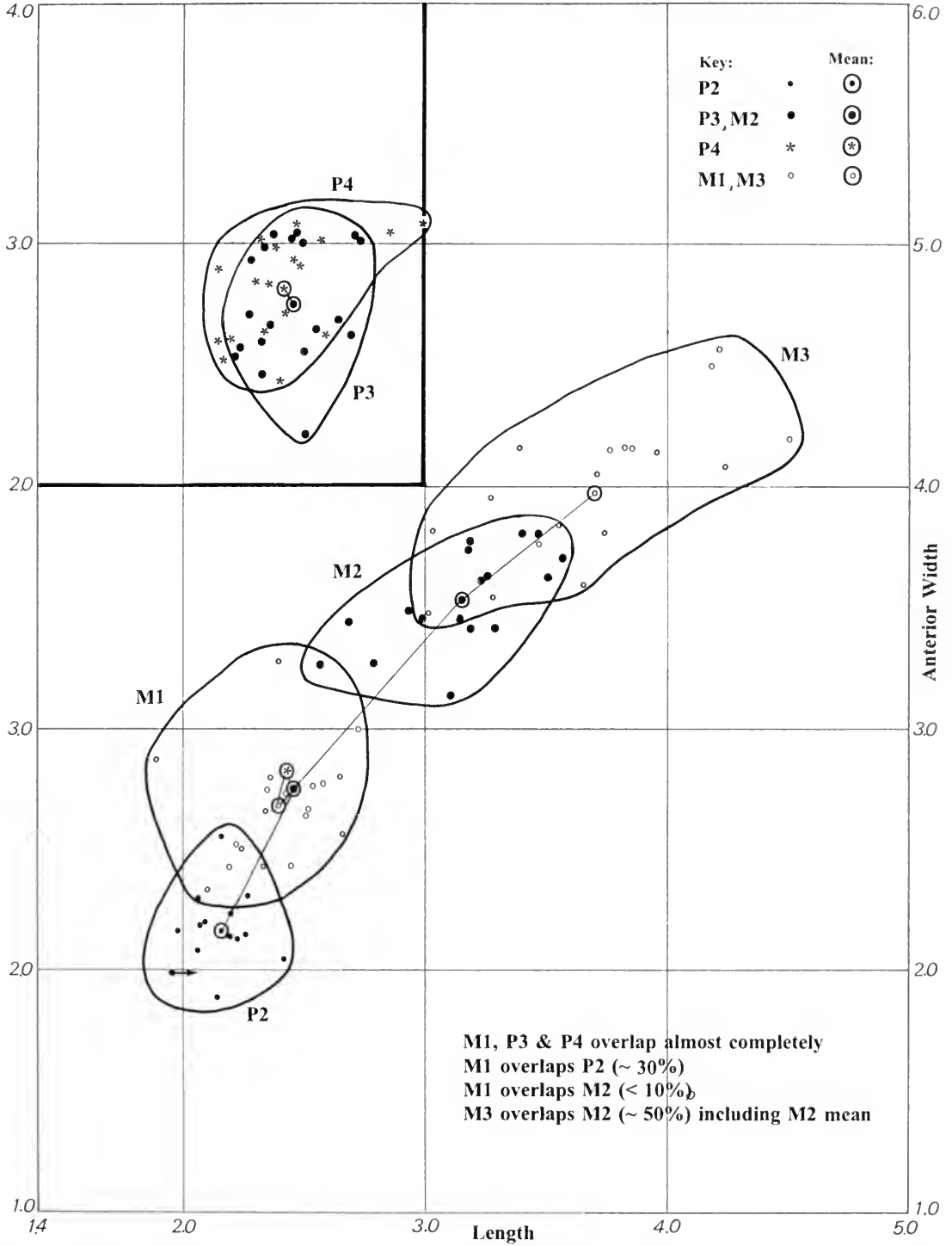
FIG. 25. Bivariate graphs for each cheek-tooth position for length × anterior width in the U. anceps upper dentition. Units are cm.
