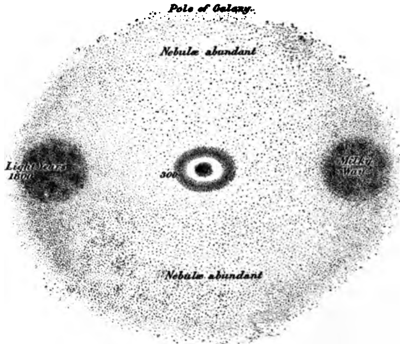
Section through Poles of Milky Way.
