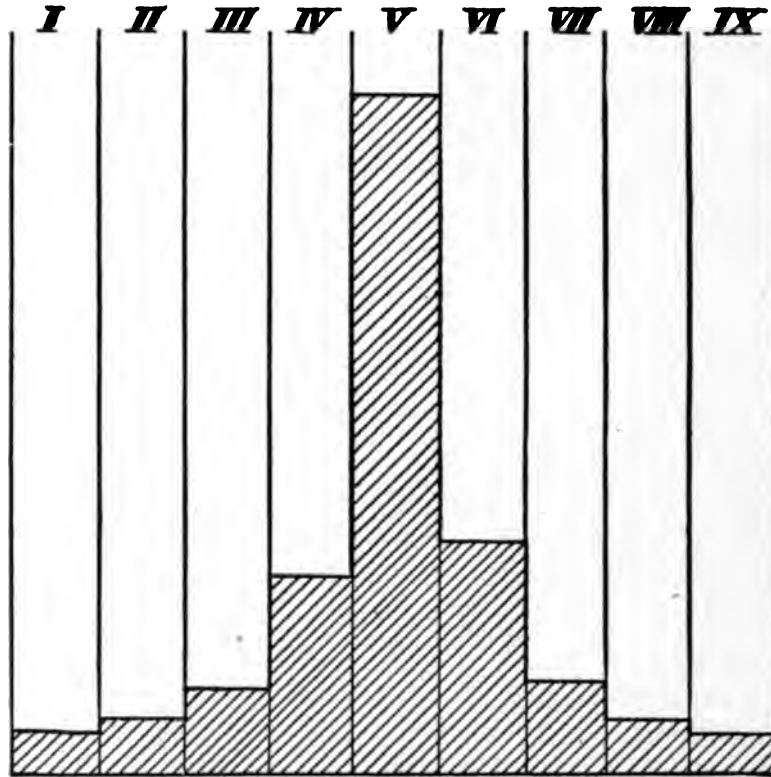
DIAGRAM OF STAR-DENSITY
