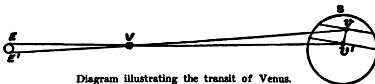
Diagram illustrating the transit of Venus.
