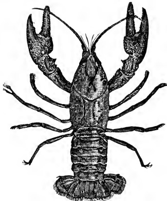
FIG. 3.—A Cray-fish.
