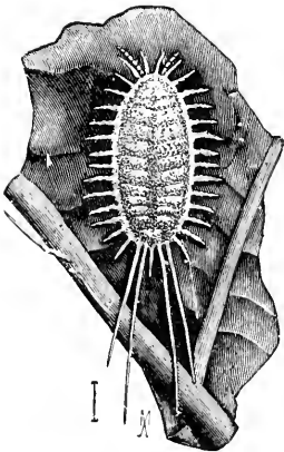
FIG. 202. — Pseudococcus longispinus , female, enlarged.
