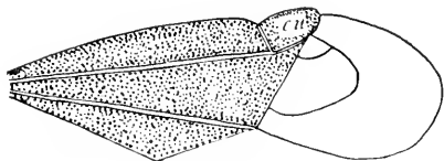
FIG. 148. — Diagram of a front wing of a mirid: cu , cuneus.
