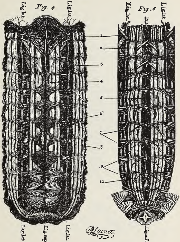
INTERNAL ANATOMY OF A CATERPILLAR ( Cossus ligniperda ).
