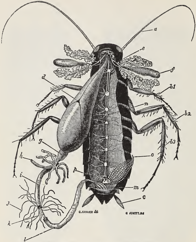
INTERNAL ANATOMY OF A COCKROACH ( Periplaneta orientalis ).
