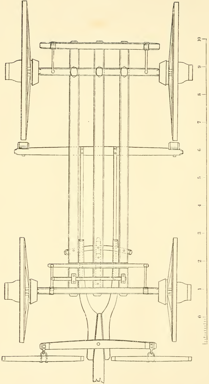
Scale of Feet. CARRIAGE-PART OF CONCORD COACH.
