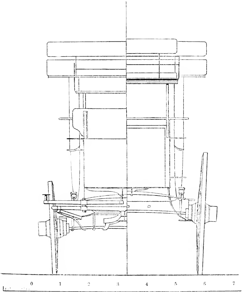
Scale of Feet. FRONT VIEW. REAR VIEW.
