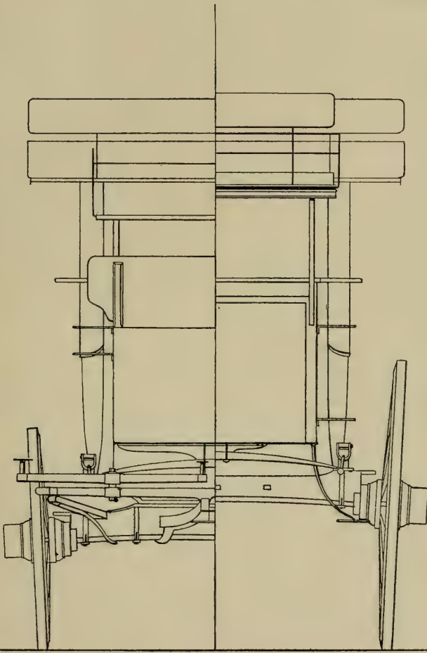
Scale of Feet. FRONT VIEW. REAR VIEW.
