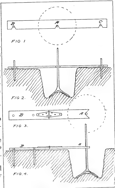
Fig. 77.—Shows two planting boards.
