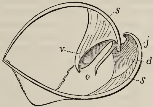
Fig. 142. Section.
