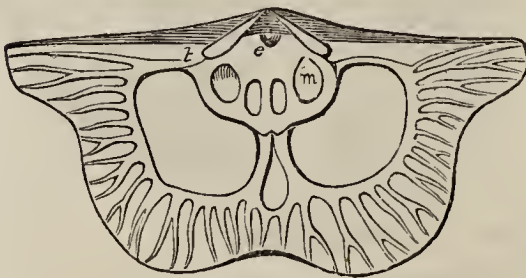
Fig. 149. Ventral valve .
