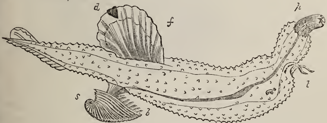
Fig. 59. A nucleobranche .*
