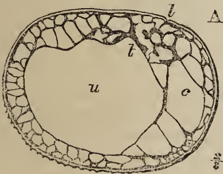
Fig. 208. Straight valve.
