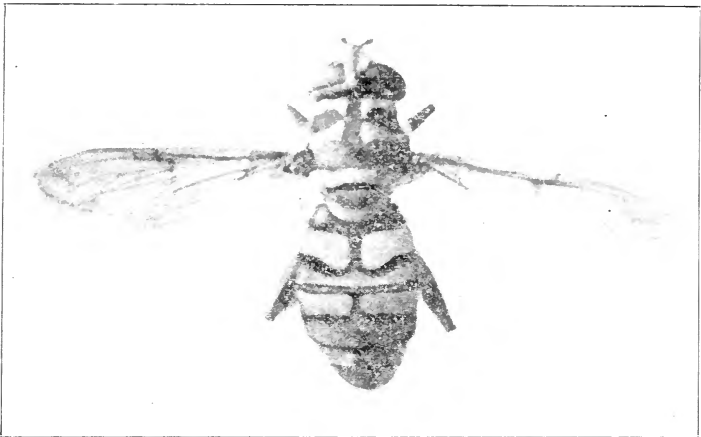
Fig. 98. Milesia virginiensis , enlarged.
