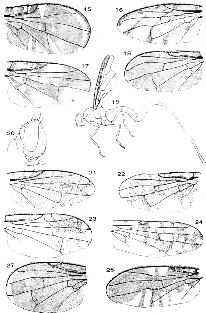
Figs. 112, 113. Trypetidae. 1, Icterica ; 2, Carphotricha ; 3, Euresta ; 4, Eutreta ; 5, Urellia ; 6, Tephritis ; 7, Oedaspis ; 8, Neospilota ; 9, Herachata ; 10, Straussia ; 11, Anastrepha ; 12, Oedicarena ; 15, Polymorphomyia ; 16, Plagiotoma ; 17, Xenochata ; 18, Eurosta ; 19, Toxotrypana (Snow); 20, Anastrepha , head; 21, Euresta ; 22, Eurosta ; 23, Urellia ; 24, Ensina ; 26, Aciura ; 27, Eutreta . (27)
