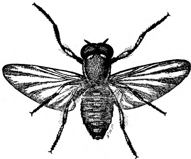
Fig. 44. Simulium venustum , enlarged. After Washburn.
