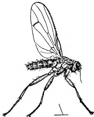
Fig. 130. Leria pubescens , enlarged. After Washburn.
