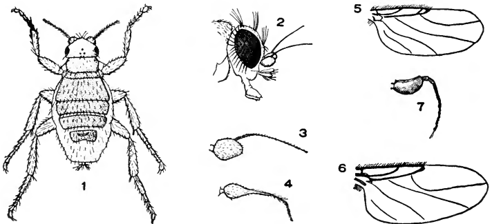
Fig. 91. Phoridae. 1, Puliciphora ♀; 2, Aphiochata , head; 3, Phora , antenna; 4, Conicera , antenna; 5, Aphiochata , wing; 6, Hypocera , wing; 7, Apocephalus , antenna. Drawings by Mrs. C. T. Brues.
