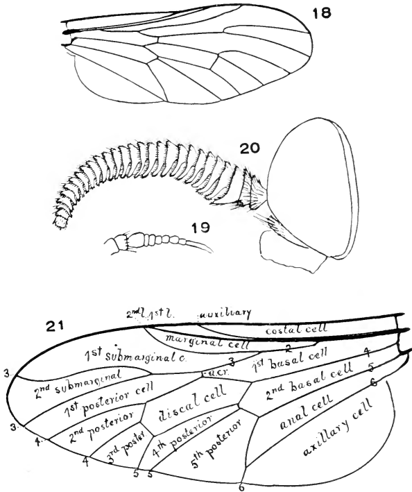
Fig. 54. Leptidæ. 18, Arthroceras (type), wing; 19, Arthroceras (type), antenna; 20, Rhachicerus , head; 21, Atherix , venation.
