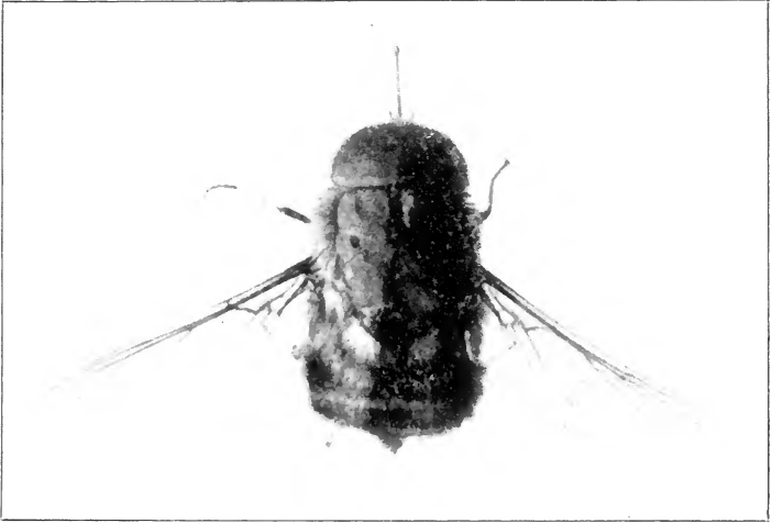
Fig. 69. Trichophthalma , species (Nemestrinidæ); enlarged.
