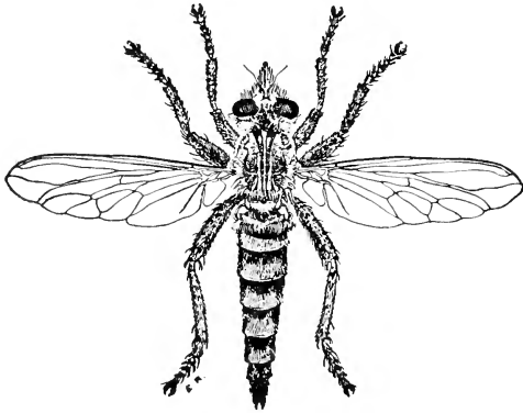
Fig. 75. Promachus vertebratus , natural size. After Washburn.
