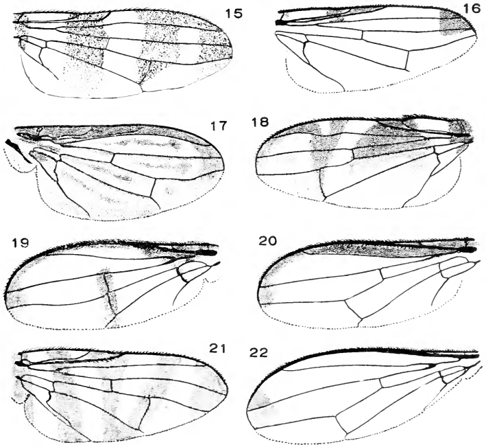
Figs. 108, 109. Ortalididæ. 1, Pyrgota ; 2, Stenopterina ; 3, Camp-toneura ; 4, Idana ; 5, Rivellia ; 6, Tetanops ; 7, Pseudotephritis ; 8, Oedopa ; 9, Chetopsis ; 10, Celometopia ; 11, Pterocalla ; 12, Melie-ria ; 13, Eumetopia ; 14, Richardia ; 15, Euxesta ; 16, Euxesta ; 17, Notogramma ; 18, Euphara ; 19, Antineura ; 20, Gen. nov? 21, Apospasmica ; 22, Stenomacra .
