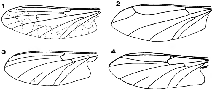
Fig. 47. Blepharoceridæ. 1, Blepharocera , wing, showing secondary venation (Comstock); 2, Paltostoma schineri , wing; 3, Phylorus , wing (Kellogg); 4, Bibiocephala , wing (Kellogg).
