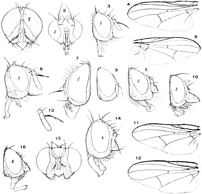
Fig. 136. Anthomyiidae. 1, Hyetodesia ( Phaonia ) lucorum , head, from front; 2, Schænomyza chrysostoma , head, from in front; 3, Cænoscia cinerea , head; 4, Lasiops spiniger , wing; 5, Lasiops spiniger ; head; 6, Phyllogaster cordyluroides , head; 7, Homalomyia ( Fannia ) scalaris head; 8, Homalomyia scalaris , wing; 9, Ophyra aenescens , head; 10, Spilogaster , species, head; 11, Spilogaster , wing; 12, Leucomelina , species, wing; 13, Leucomelina , antenna; 14, Lispa uliginosa , head; 15, Lispa , species, head from in front; 16, Limophora exul , head.
