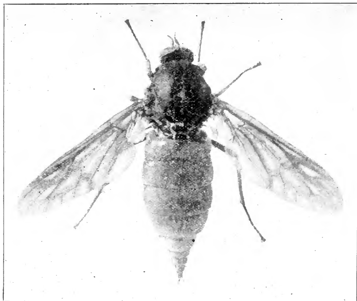
Fig. 52. Ctenomyia ferruginea , female; enlarged.
