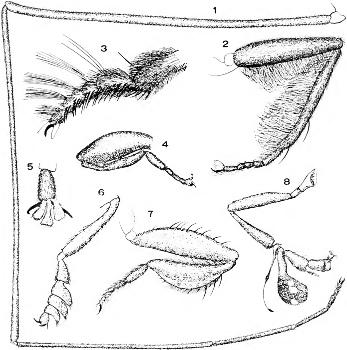
Fig. 9. Legs. 1, leg of Tipulid; 2, middle leg of Peckia praecipis , male; 3, hind foot of Mallophora scopipeda , male; 4, hind leg of Tropidia quadrata ; 5, last tarsal joint of Dialysis ; 6, front leg of Stegana horca , male; 7, hind leg Rhopalomera ciliata ; 8, hind leg of Calotarsa , male.
