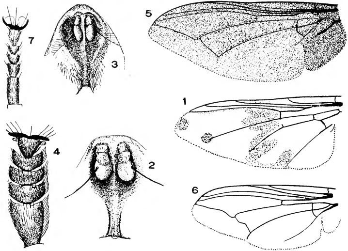
Fig 141. Æstridæ . 1, Gastrophilus , wing; 2, Gastrophilus , antennæ; 3, Cuterebra , antennæ; 4, Cuterebra , front tarsus; 5, Cuterebra , wing; 6, Dermatobia , wing; 7, Dermatobia , front tarsus.
