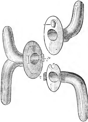
FIG. 425.—Vachette's Tube.
