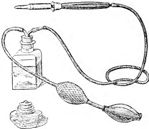
FIG. 214.—Paquelin Cautery.
