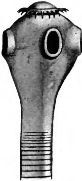
FIG. 69.—Head of Tania solium , magnified. (After Leuckart.)
