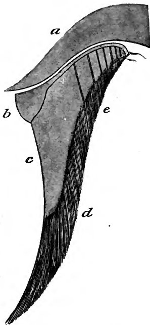
FIG. 299.—Section of upper jaw, (a), with baleen-plates, of Balænoptera . (After Owen.)
