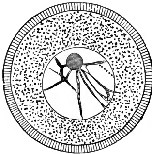
FIG. 25.—Ovum of a Sea-Urchin, showing the radially striated cell-membrane, the protoplasm, containing yolk-granules, the large nucleus (germinal vesicle), with its network of chromatin and a large nucleolus (germinal spot). (From Bal-four's Embryology , after Hertwig.)
