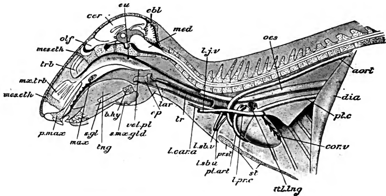
FIG. 282.— Lepus cuniculus . Lateral dissection of the head, neck and thorax. The head and spinal column are represented in mesial vertical section; the left lung is removed; the greater part of the nasal septum is removed so as to show the right nasal cavity with its turbinals. aort. dorsal aorta; b. hy. basi-hyal; cbl. cerebellum; cer. cerebral hemispheres; cor. v. coronary vein; dia. diaphragm; ep. epiglottis; eu. opening of Eustachian tube into pharynx; lar. larynx; l. j. v. left jugular vein; l. sb. a. left subclavian artery; l. sb. v. left subclavian vein; med. medulla oblongata; mes. eth. mesethmoid; mx. trb. maxilla-turbinal; æs. oesophagus; olf. olfactory lobe; pl. art. pulmonary artery; p. max. pre-maxilla; pr. st. pre-sternum; pl. c. post-caval vein; rt. l. lng. root of left lung with bronchus and pulmonary veins and artery cut across; s. gl. sub-lingual salivary gland; s. mx. gl. sub-maxillary salivary gland; st. sternæbræ; tng. tongue; tr. trachea; trb. ethmo-turbinals; vel. pl. soft palate.
