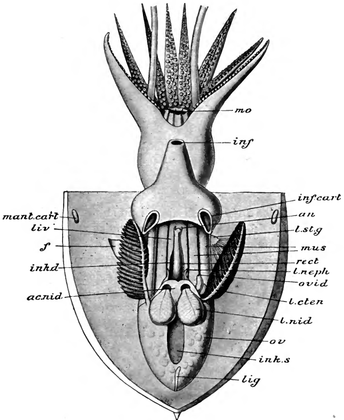
FIG. 178.— Sepia cultrata , female seen from the posterior aspect, the wall of the mantle-cavity divided along the middle line and the two flaps thus formed spread out so as to expose the contents. ac. nid. accessory nidamental glands; an. anal aperture with its lateral appendages; f. membranous fold attaching the ctenidium to the wall of the mantle-cavity; inf. external opening of funnel; inf. cart. infundibular cartilage; ink s. ink-sac; ink d. ink-duct; lig. ligamentous band which extends from the anterior wall of the mantle cavity to the ovary, cut across; liv. liver; l. cten. left ctenidium; l. neph. left nephridial aperture; l. nid. left nidamental gland; l. st. g. left stellate ganglion; mant. cart. mantle cartilage; mo. mouth; mus. neck muscles; ov. ovary; ovid. oviduct; rec. rectum.
