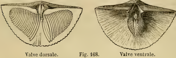
Valve dorsale.
