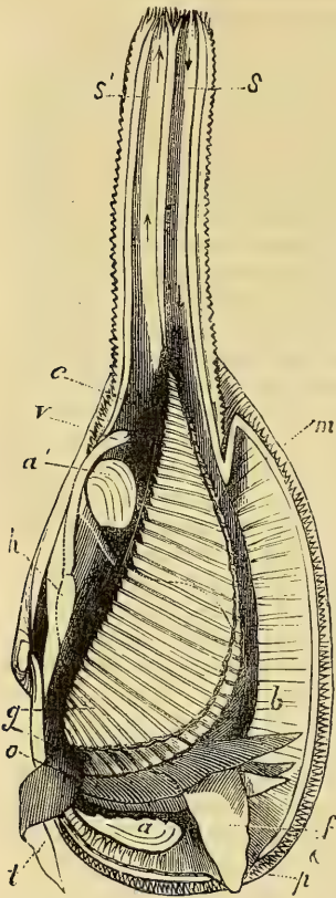
Fig. 207. — Mya arenaria 1 .
