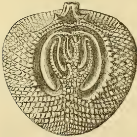
Fig. 165. — Th. radians .
