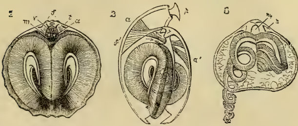
Fig. 4, 5, 6. — Brachiopodes 6 .
